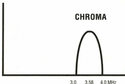
Fig. 1 Luminance and Chroma signals and their bandwidth characteristics.
