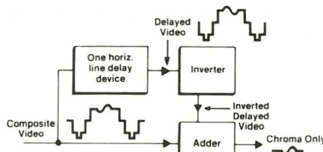
Fig. 6: Basic comb filter operation to separate luminance from the composite video signal to leave the "combed" or chroma-only signal.
