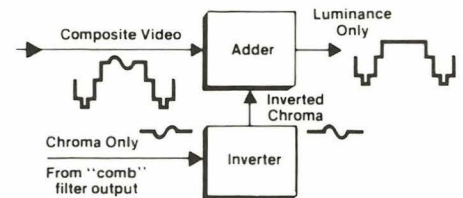
Fig. 8: By adding the "combed" chroma signal back to the original composite video signal, the two chroma signals will cancel and "comb" the chroma from the composite video signal to leave luminance without chroma.
