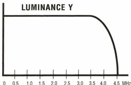
Fig. 1 Luminance and Chroma signals and their bandwidth characteristics.
