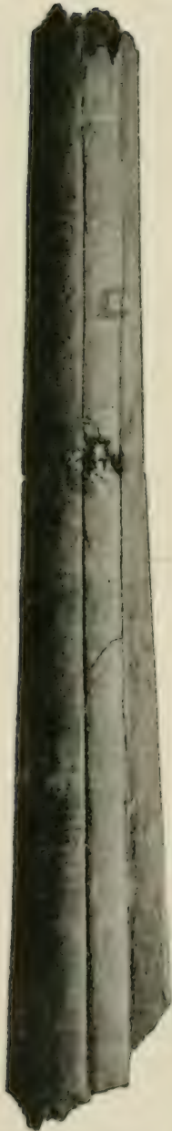
Fig. 1.—Rostrum of Priscodelphinus sp.? from the Miocene of Shiloh, N. J. Superior surface. ( \frac{1}{2} nat. size.)
