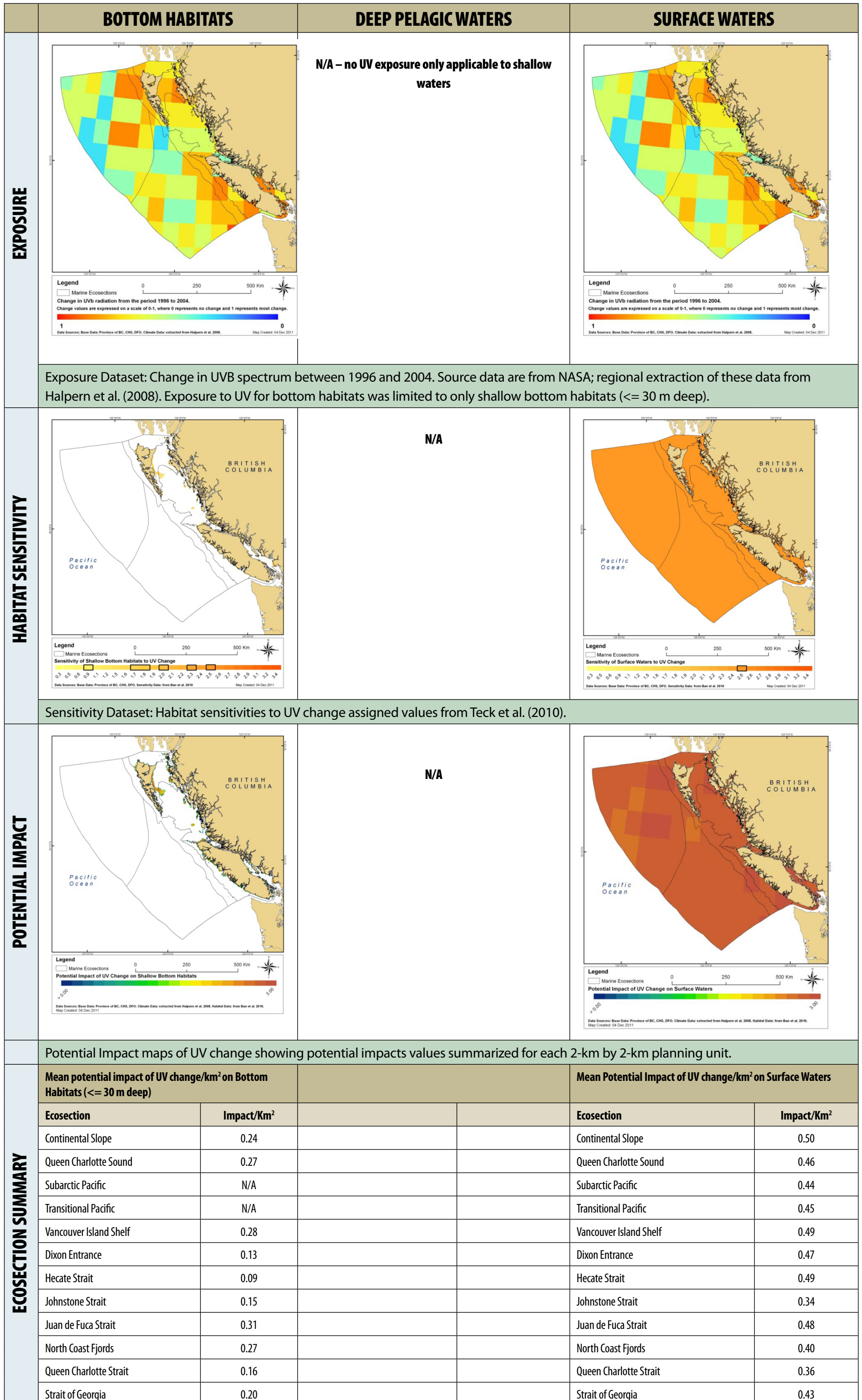
Figure 5.13 Estimate Potential Impact of UV Change calculated for the region from exposure and sensitivity maps and summarized by ecosection.
