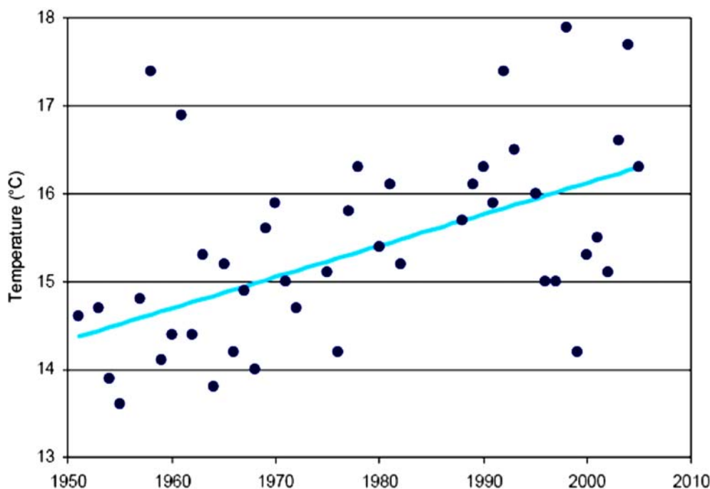
Figure 3.5 Increase in average summer (June, July, August) temperature of the lower Fraser River at Hell's Gate at the rate of 0.3 \pm 0.1^\circ\text{C} per decade since 1950. Data from the Pacific Salmon Commission and Institute of Ocean Sciences, Fisheries and Oceans Canada.
