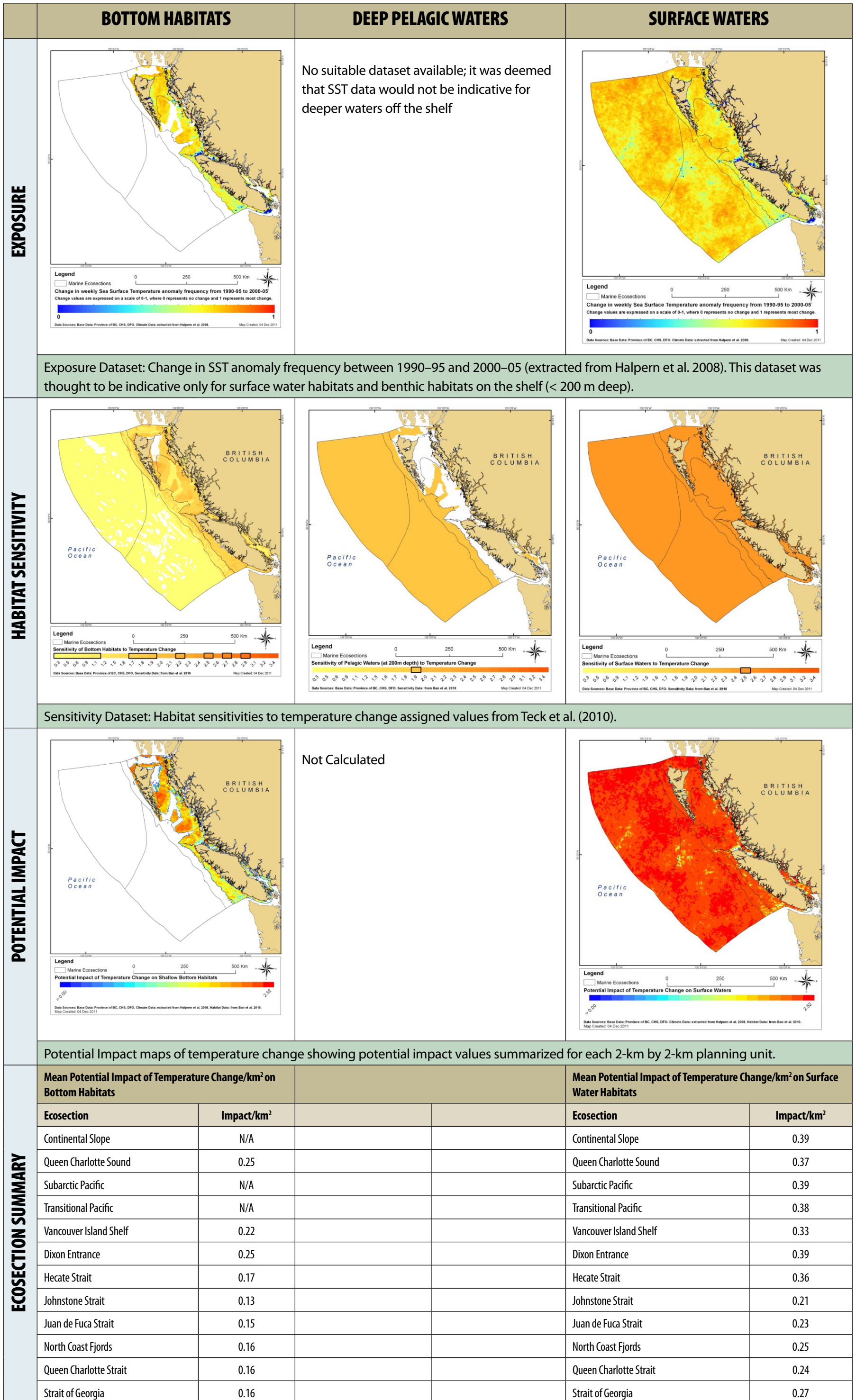
Figure 5.11 Estimated Potential Impact of Temperature Change calculated for the region from exposure and sensitivity maps and summarized by ecoregion.
