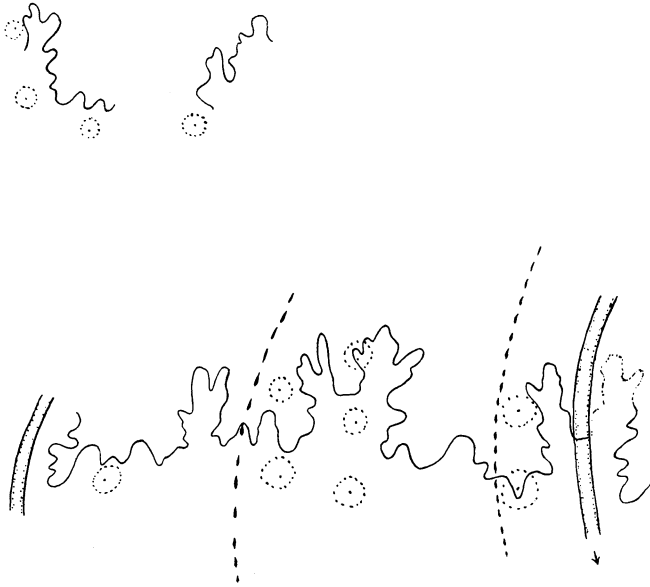
Fig. 6. Suture, Turrilites worthensis n. sp., camera lucida drawing. The upper left hand figure is from the type.
