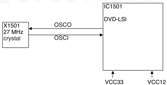
Fig 5.1: Clock configuration
