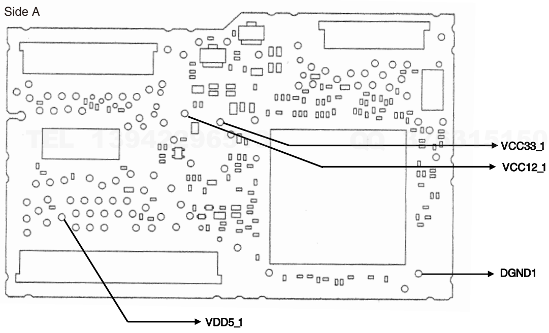
Fig 2.2: VDD5, VCC33, VCC12 voltage check points
