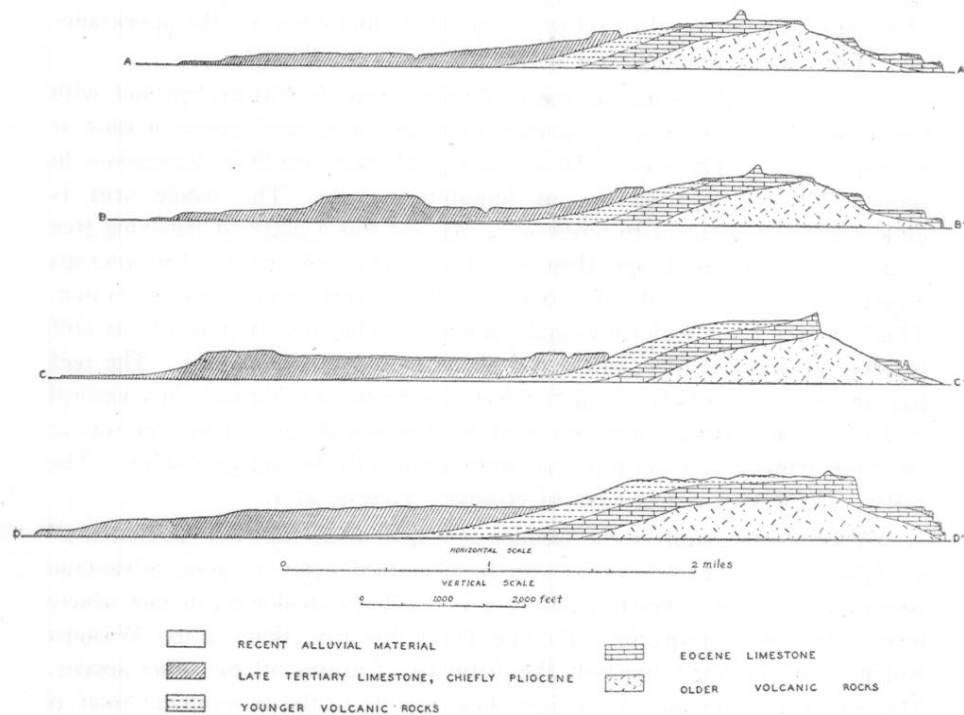
FIGURE 4.—Structure sections across Eua, along lines shown in figure 3.
