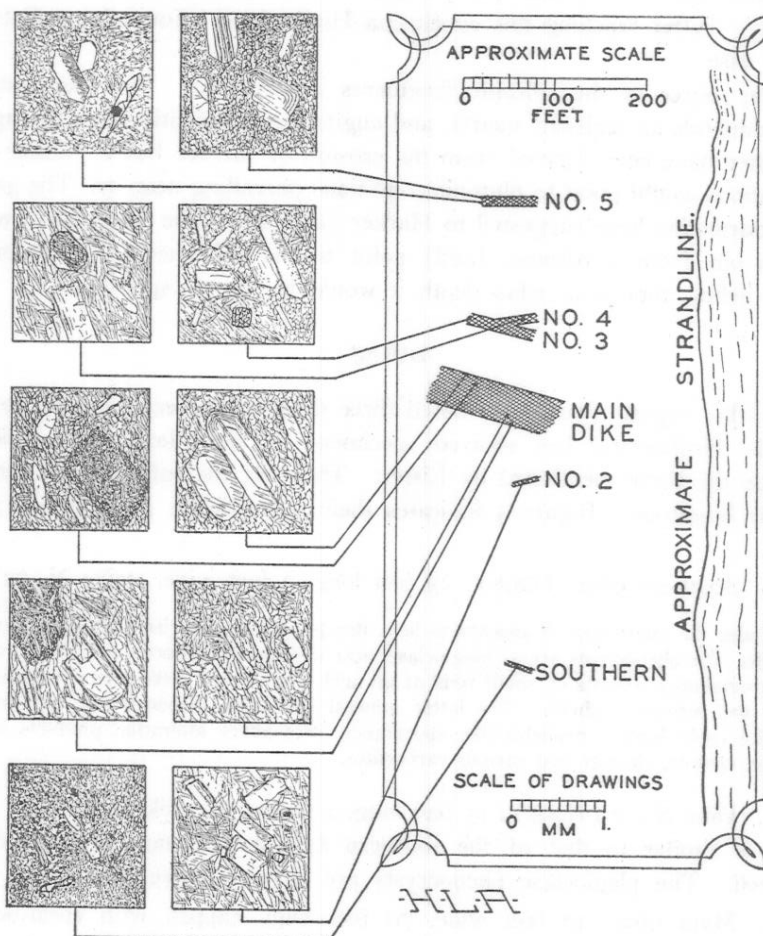
FIGURE 5.—Dikes along the east coast of Eua: right side, sketch map showing position of the dikes; left side, microscopic drawings showing petrographic character of the dike rocks, viewed in polarized light.
