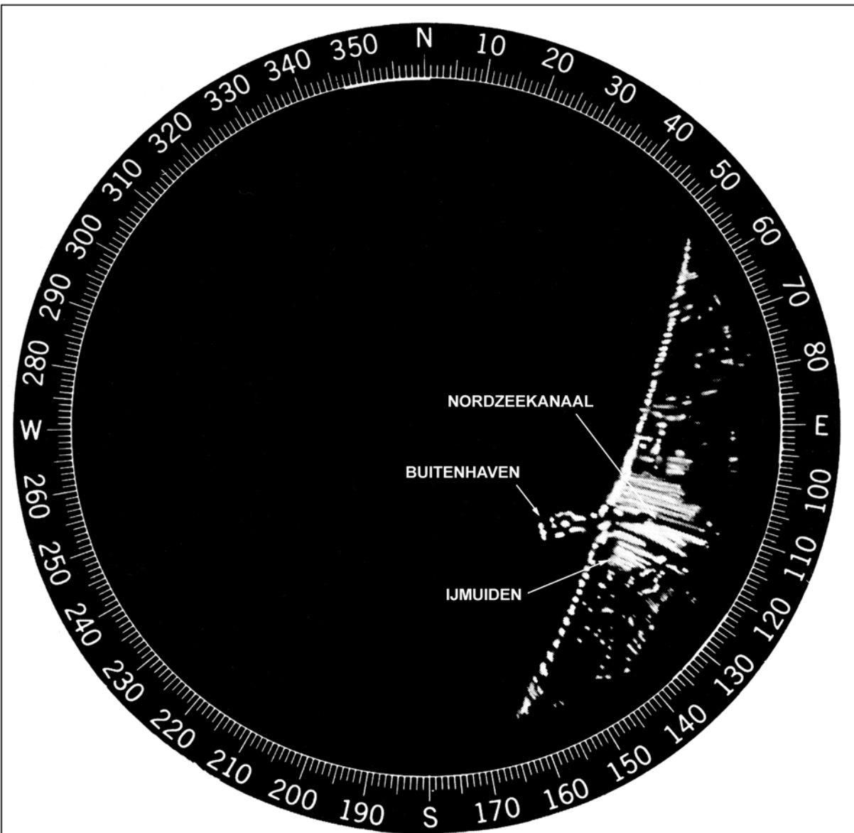
PPI DISPLAY APPROACH TO NORDZEEKANAAL (AMSTERDAM) POSITION: 52°30.0'N. 004°27.8'E. RANGE SCALE: 8M
