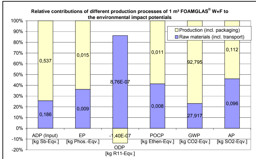
Figure 7-5: Relative contributions of different production processes of 1 m³ FOAMGLAS® W+F to the environmental impact potentials
