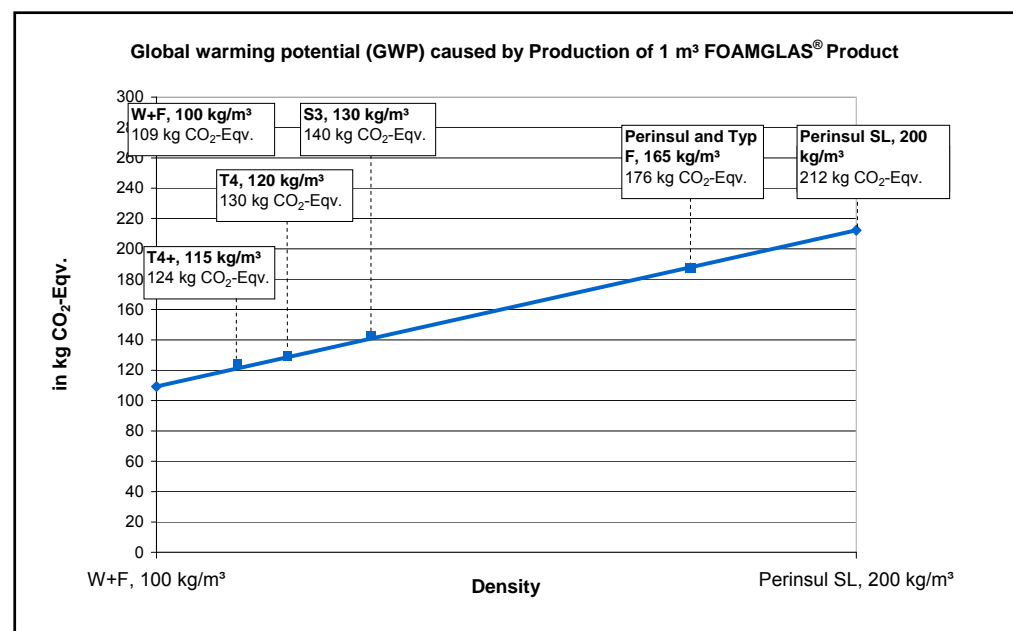
Figure 7-4: Global warming potential (GWP) caused by the production of 1 m 3 FOAMGLAS® product
