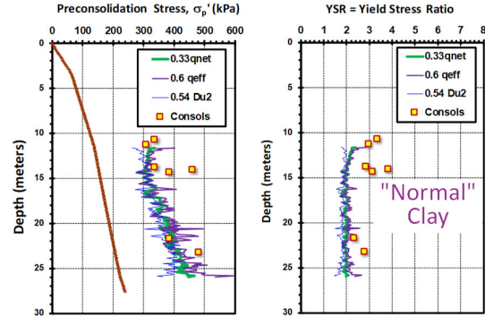
Figure 7. Screening for normal versus organic versus sensitive clays using the CPTu
