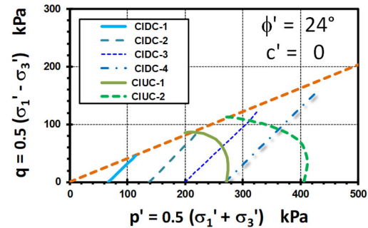
Figure 4. Triaxial strength envelopes for Hartford clay
