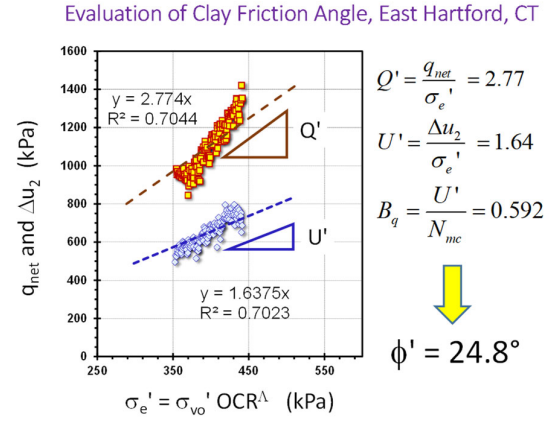
Figure 10. Post-processing of CPTu data in OC varved Hartford clay for evaluation of effective friction angle
