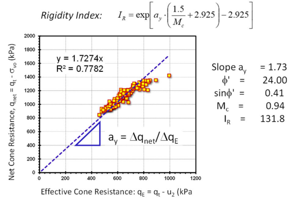
Figure 8. CPTu data analysis to determine slope parameter a_y for rigidity index
