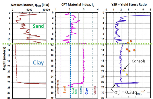
Figure 6. Profile of CPT material index and first-order estimate of yield stress in Hartford clay
