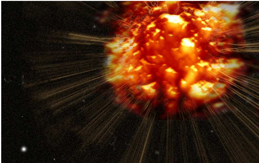
Obrázek 3: Supernova http://perspective.mit.edu/contests/2007/30/www/
