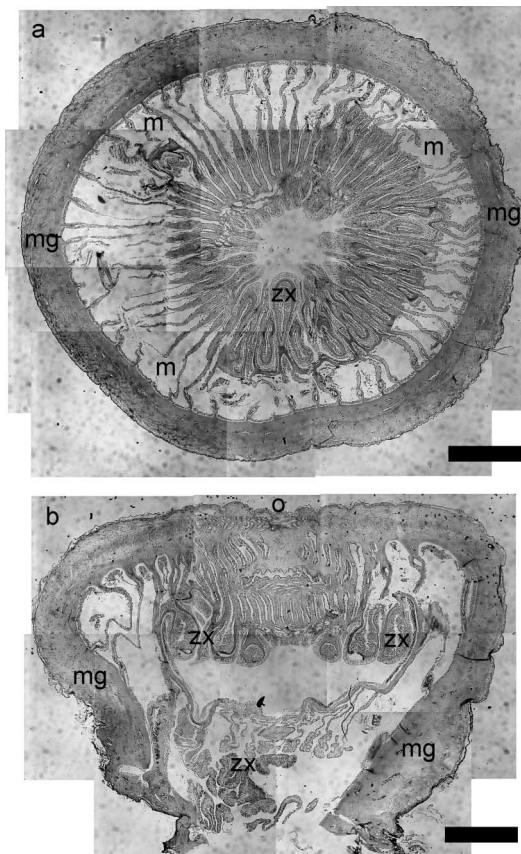
Fig. 7. Sections of Zoanthus kuroshio n. sp. a) Cross section of Z. kuroshio n. sp. showing several polyps (numbers) and a well-developed coenenchyme. b) longitudinal section of two polyps (1, 2) and coenenchyme of Z. kuroshio n. sp. Abbreviations: m, mesentery; mg, mesoglea; zx, zooxanthellae; c, coenenchyme; o, oral opening. Note that the coenenchyme consists primarily of mesoglea. All black bars=1000 \mu m. All sections from holotype colony NSMT-CO 1445.
