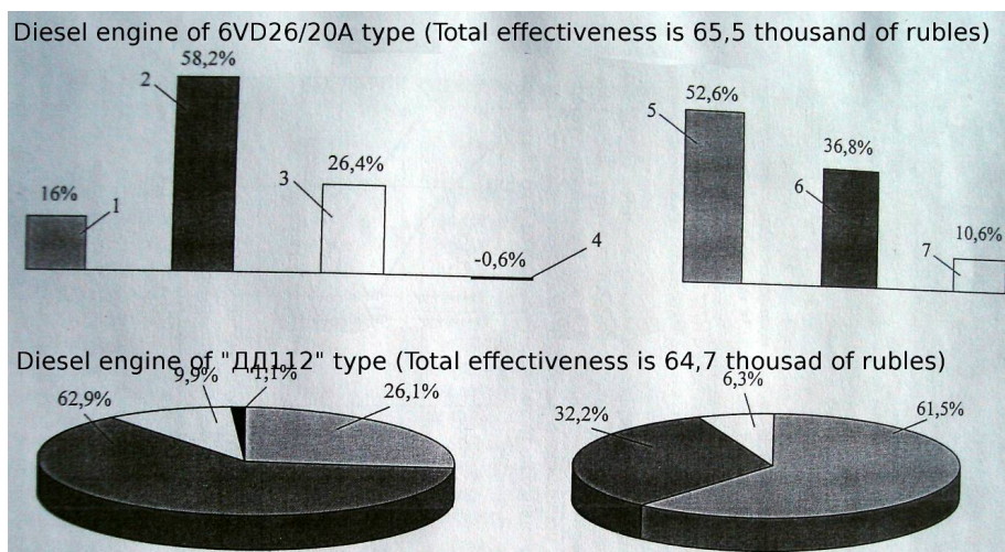
Figure 3. Cost savings at the complex improvement of lubrication systems of marine upgraded types of the diesel engines: 1—overhaul; 2— engine cleaning, 3—Oil, 4—filter elements, 5—oil (additives), 6—oil cleaning complex; 7—elements of the lubrication system.
