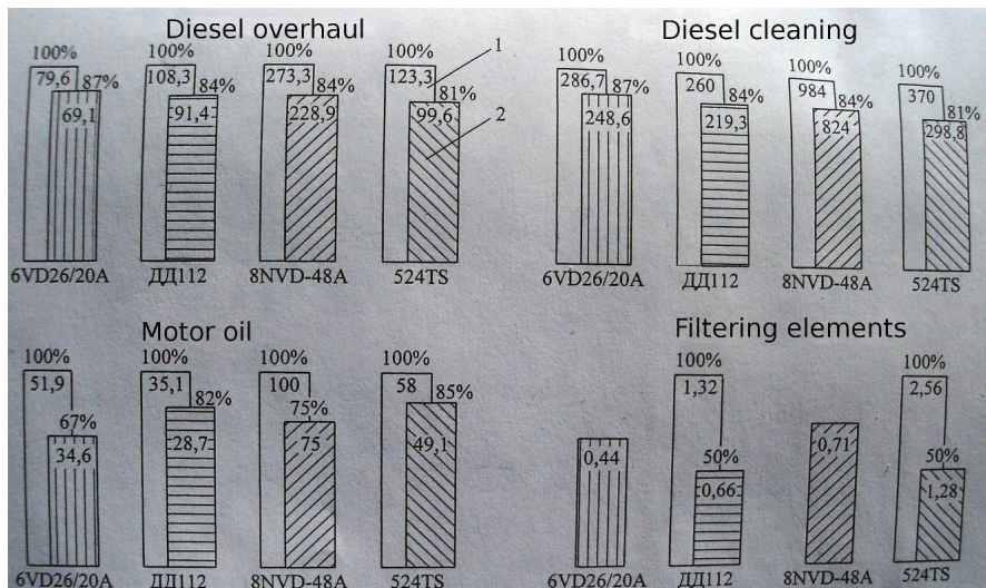
Figure 1. Annual operating (conditional) costs (thousand of rubles) of the of trunk piston diesel engines maintenance with standard (1) and upgraded (2) lubrication systems.
