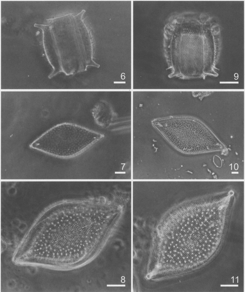
Figs 6–11. Odontella atlantica , light microscope, phase contrast. Figs 6–8. Specimen and valves found in slide 167 (3) from Mar del Plata, Argentina, in Frenguelli Collection. Fig. 6. Frustule. Figs 7, 8. Valvar views. Figs 9–11. Specimen and valves found in Santa Teresita. Fig. 9. Frustule. Figs 10, 11. Valvar views. Scale bars = 10 \mu\text{m} (Figs 6–11).
