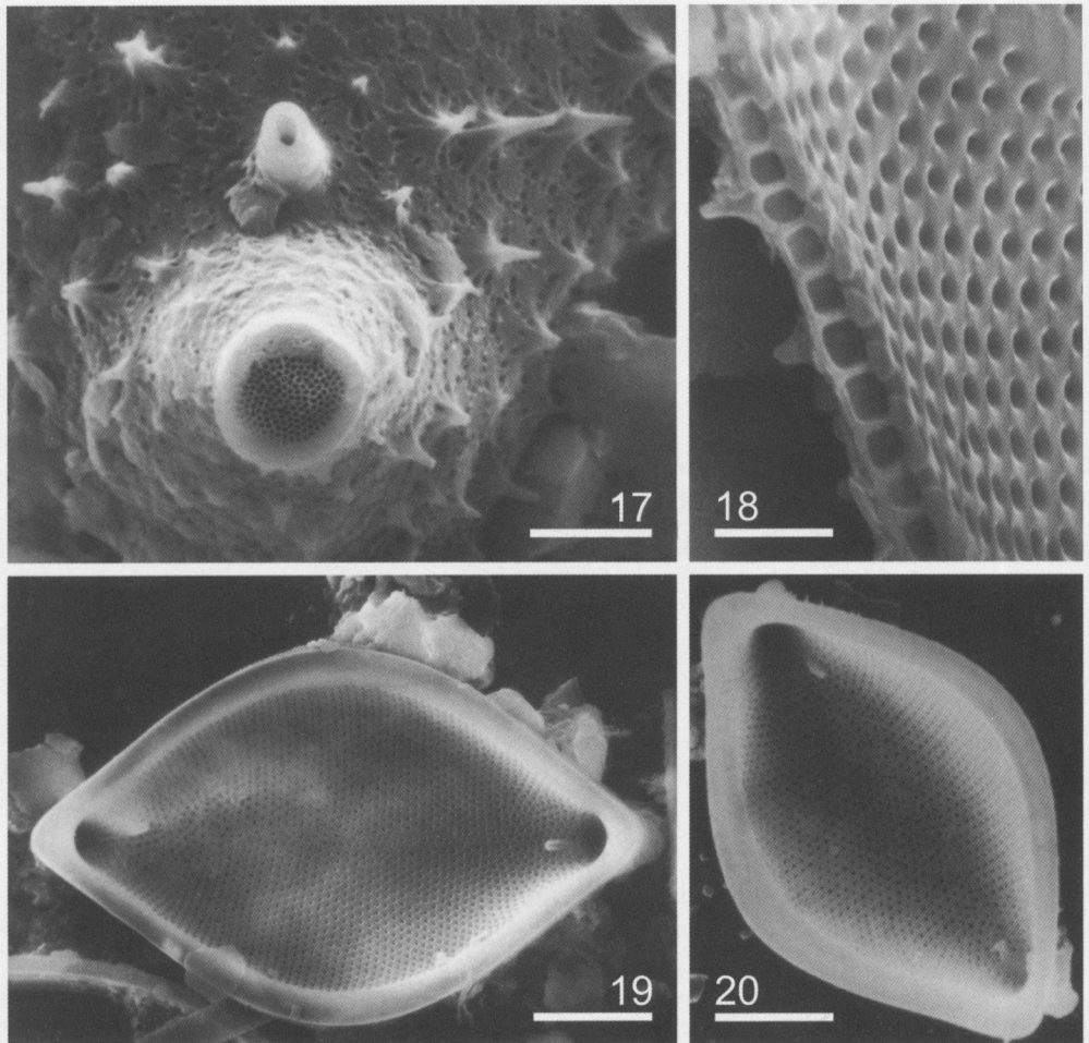
Figs 17–20. Odontella atlantica , scanning electron microscopy. Fig. 17. Valve found in Santa Teresita. Elevation with ocellus showing porelli. Note imperforated velum with several holes around the periphery and buttressed spines. Fig. 18. Valve found in Mar de Ajó. Broken valve showing loculate areolae with internal foramen and external velum. Figs 19, 20. Valves found in San Clemente del Tuyú and Villa Gesell respectively. Valves in internal view. Note pattern of striation and sessile lips of the labiate processes in almost apical position. Scale bars = 2 \mu\text{m} (Figs 17, 18); 10 \mu\text{m} (Figs 19, 20).
