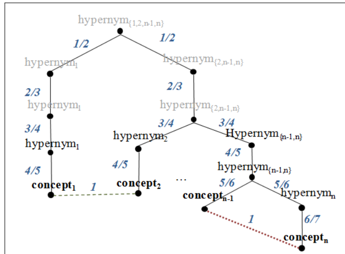
Figure 4.4: Document graph (Jaccard coefficient)
