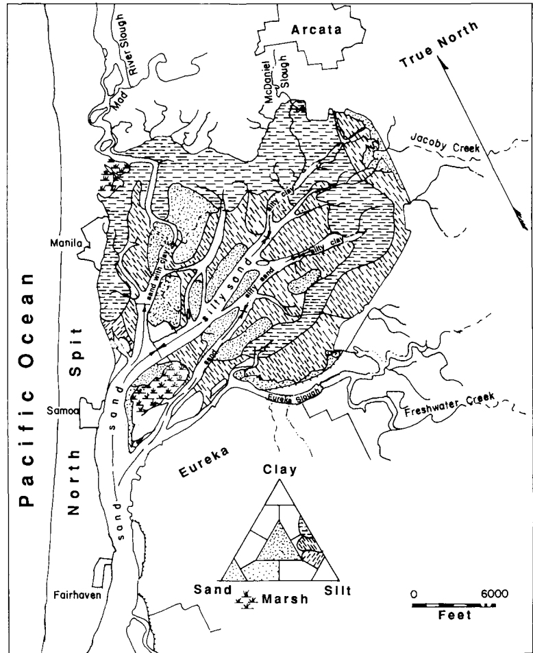
Fig. 2.2. Sediment distribution in Arcata Bay (from Thompson 1971).
