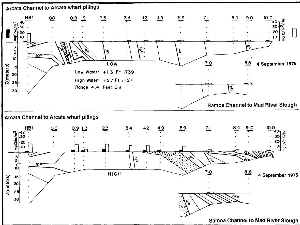
Fig. 2.11. Temperature, chlorophyll (black bar), and productivity distribution (white bar) at low and high tides in channels from Humboldt Bay entrance into Arcata Bay, 4 September 1975. Station HB1 is marker buoy 1 nmi off shore; station 0.0 is at mouth of Humboldt Bay; and all other stations are indicated by distance in nautical miles up bay from mouth (Pequegnat and Butler 1982).
