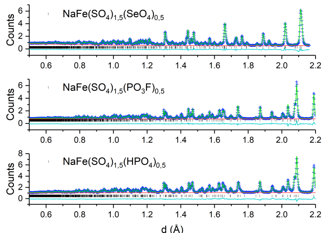
Figure 2: Observed, calculated and difference profiles from Rietveld refinement using ND data for \text{NaFe}(\text{SO}_4)_{1.5}(\text{X})_{0.5} ( \text{X} = \text{SeO}_4, \text{HPO}_4, \text{PO}_3\text{F} )
