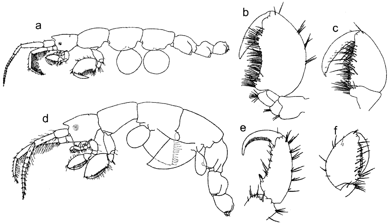
Figure 10. Caprella penantis Leach, 1814, a–c, male, d–f, female; a, lateral view; b, gnathopod 2; c, gnathopod 1; d, lateral view; e, pereopod 7; f, gnathopod 2. (a–c, from McCain 1968: Figure 4; d–f, from McCain 1968: Figure 5)
