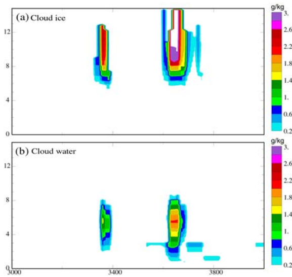
Fig. 6 West-East cross section of analyzed cloud water and cloud ice from all observations, but without a background field. The cross section is through the section that has the maximum hail mixing ratio.
