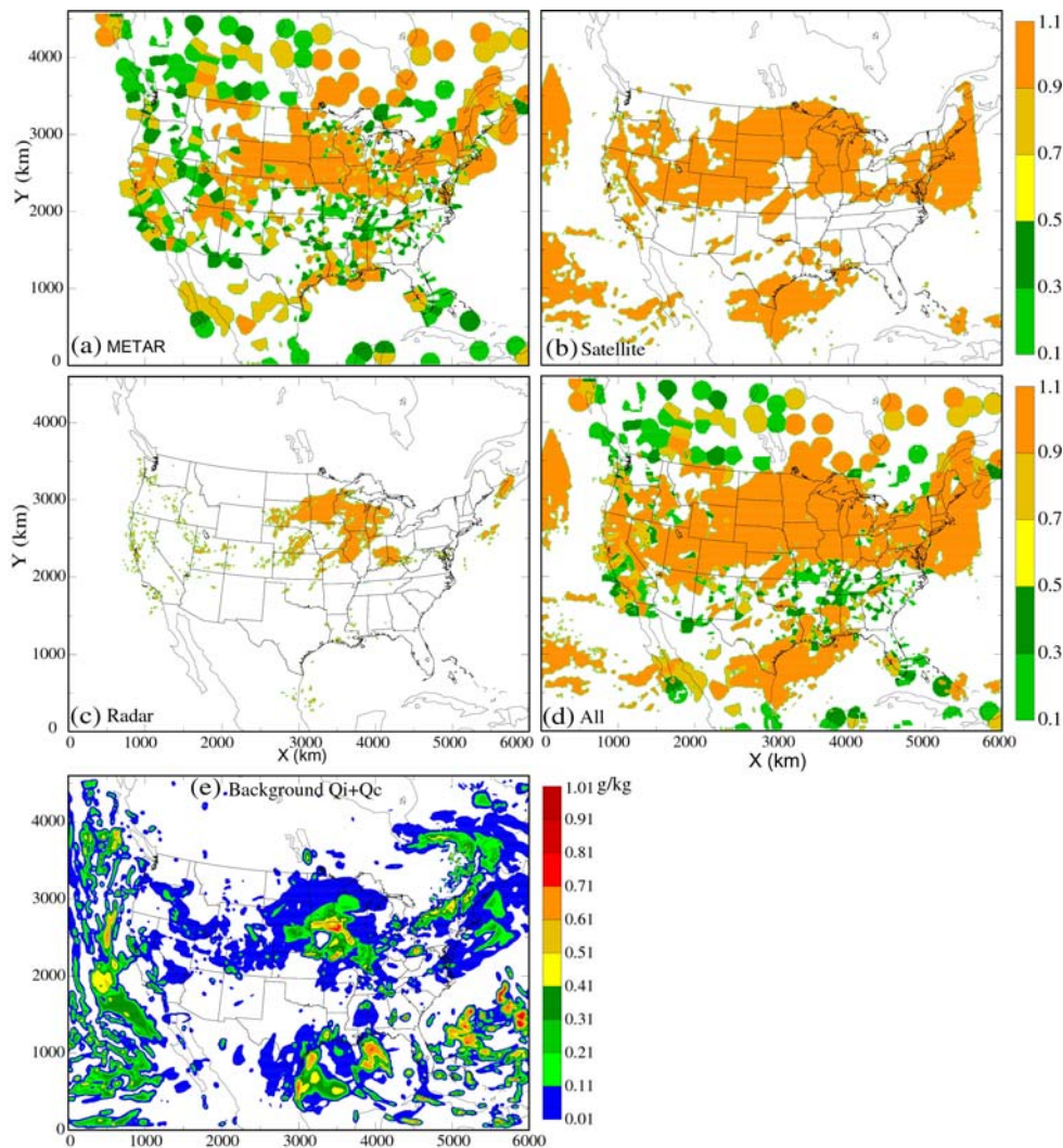
Fig. 3. Composite cloud cover (column maximum) indicated from various observations in the generalized cloud analysis: (a) METAR data only, (b) Satellite (NESDIS cloud products) only, (c) radar (NSSL mosaic reflectivity) only, and (d) all the above three data sources. e) background (1-h model forecast) cloudwater + cloud ice field.
