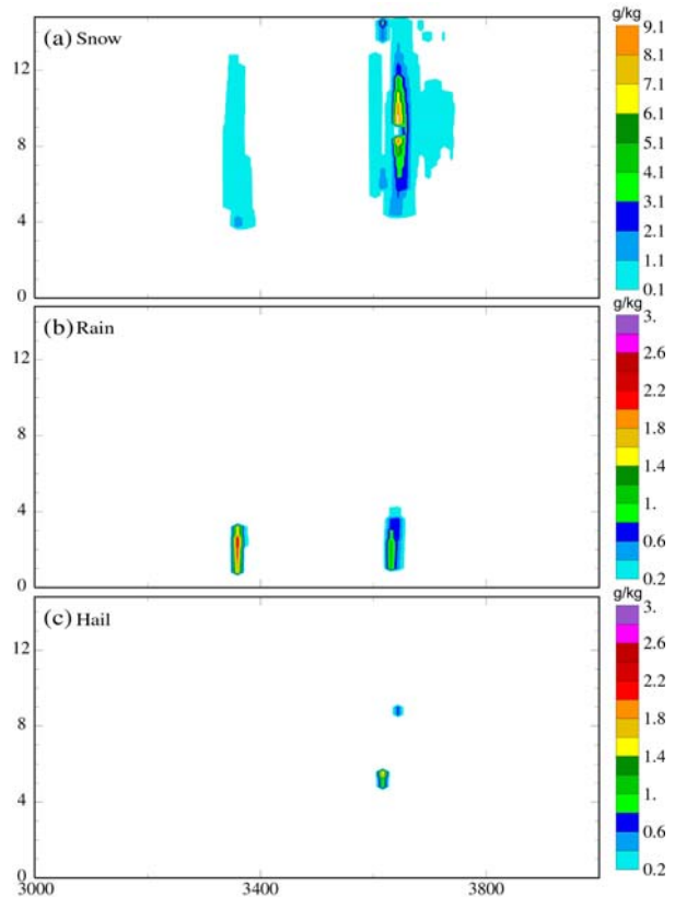
Fig. 7 West-East cross section of rain, snow, and hail deduced from all the observations. The cross section is picked to through the section that has maximum hail mixing ratio.
