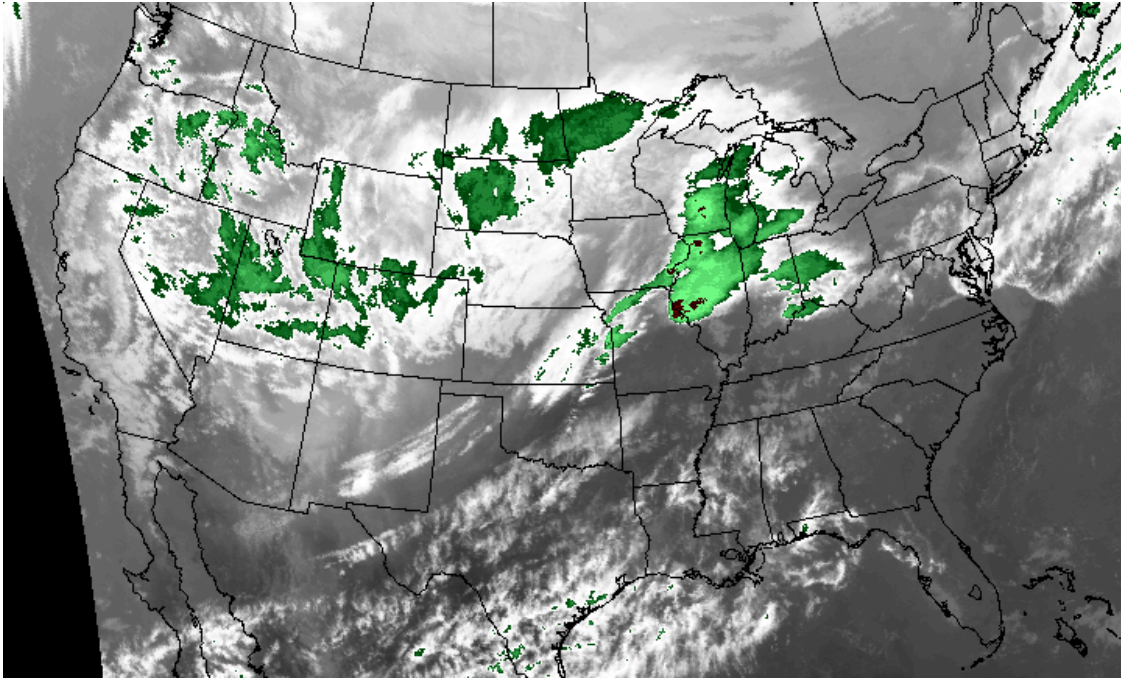
Fig. 2 GOES12 IR observation at 0015 UTC 13 March 2006.
