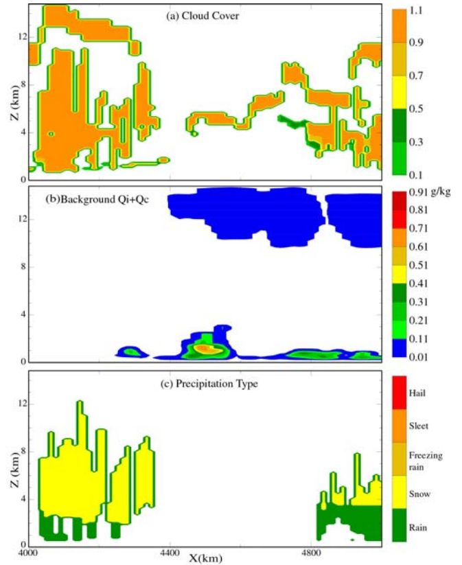
Fig. 5 Zoomed in west-east cross section of a) cloud cover deduced from all observations, b) the background cloud water and cloud ice fields and c) precipitation type deduced from the radar data and background temperature field. In a), regions where cloud cover is unknown are not indicated.
