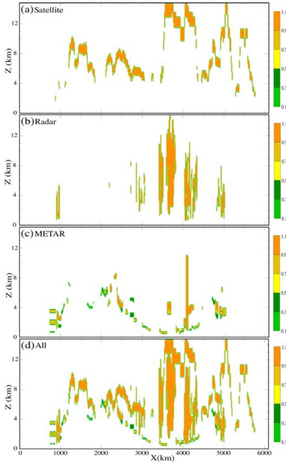
Fig. 4 West-East cross section of the analyzed cloud cover along the center of each panel in Fig. 3
