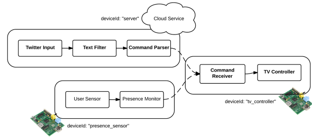
Figure 7. In a distributed flow, nodes may be hosted on servers and devices; remote wires connecting devices to servers, indicated by the dashed connections.
