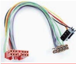
19455 ISO -> RENAULT
