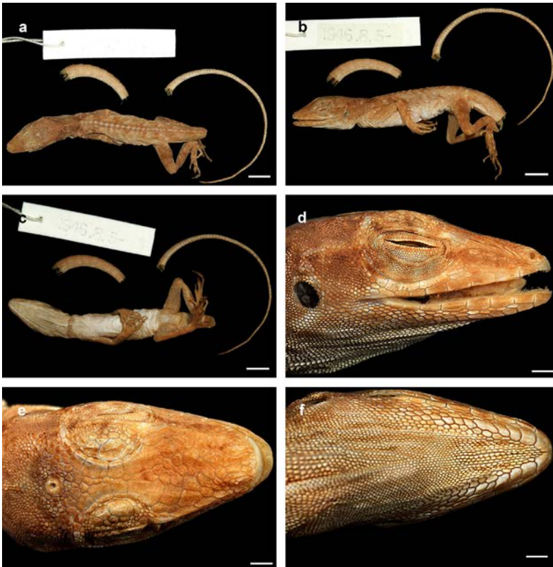
Figure 9. Holotype of Anolis citrinellus Cope, 1864 (BMNH 1946.8.5/1): (a) dorsal view; (b) lateral view; (c) ventral view; (d) lateral view of head; (e) dorsal view of head; (f) ventral view of head. Scale bars equal 5.0 mm in (a–c) and 1.0 mm in (d–f), respectively. Photos by Gunther Köhler.
