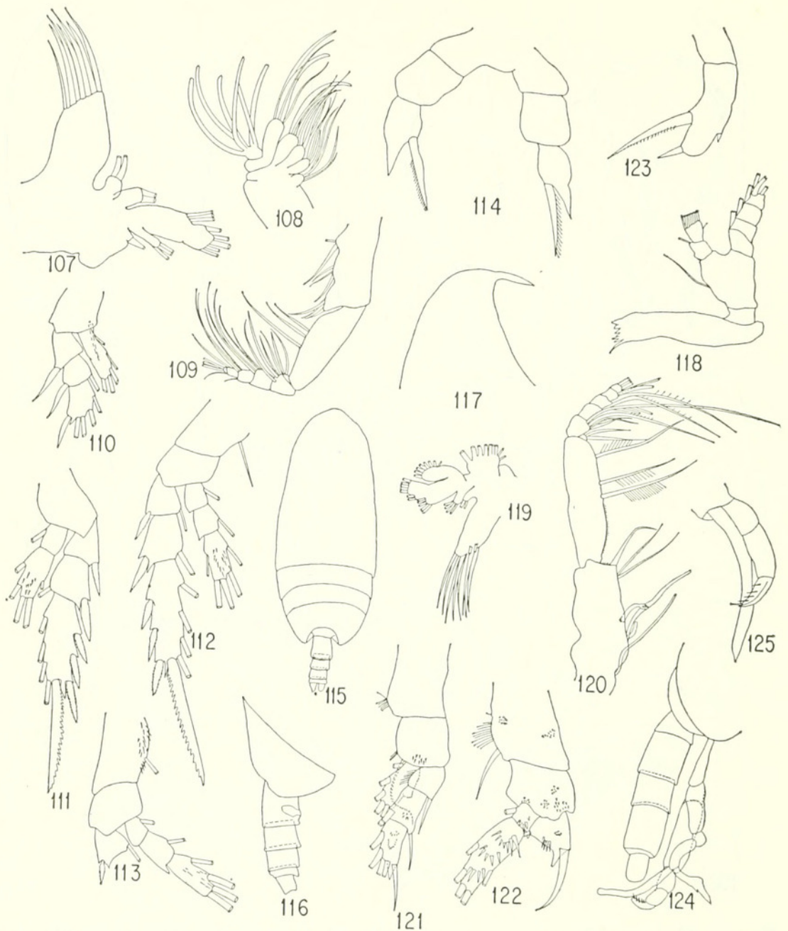
FIGURES 107-125.— Scolecithricella maritima , new species, female: 107, first maxilla; 108, second maxilla; 109, maxilliped; 110, first foot; 111, second foot; 112, third foot; 113, fourth feet (second and third exopodal segments broken off); 114, fifth feet. Scolecithricella timida , female: 115, dorsal view; 116, fourth and fifth thoracic segments and abdomen, lateral view; 117, anterior end of head, lateral view; 118, mandible; 119, first maxilla; 120, maxilliped; 121, first foot; 122, second foot (second and third exopodal segments broken off); 123, fifth foot. Scolecithricella , species, male: 124, abdomen and fifth feet, lateral view; 125, distal end of left fifth foot (enlarged).
