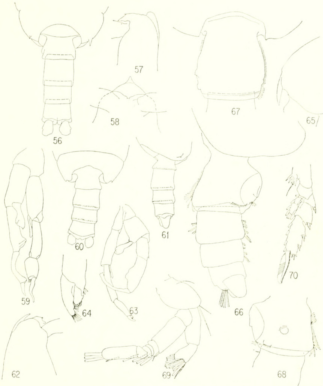
FIGURES 56-70.— Gaetanus ferox , male: 56, fifth thoracic segment and abdomen, dorsal view; 57, anterior end of head, lateral view; 58, anterior end of head, ventral view; 59, fifth feet. Gaidius robustus , male: 60, fifth thoracic segment and abdomen, dorsal view; 61, fifth thoracic segment and abdomen, lateral view; 62, anterior end of head, lateral view; 63, fifth feet; 64, distal end of left fifth foot. Pseudochirella squalida , new species, female: 65, anterior end of head, lateral view; 66, abdomen, lateral view; 67, genital segment, dorsal view; 68, genital segment, left side; 69, second antenna; 70, fourth foot.
