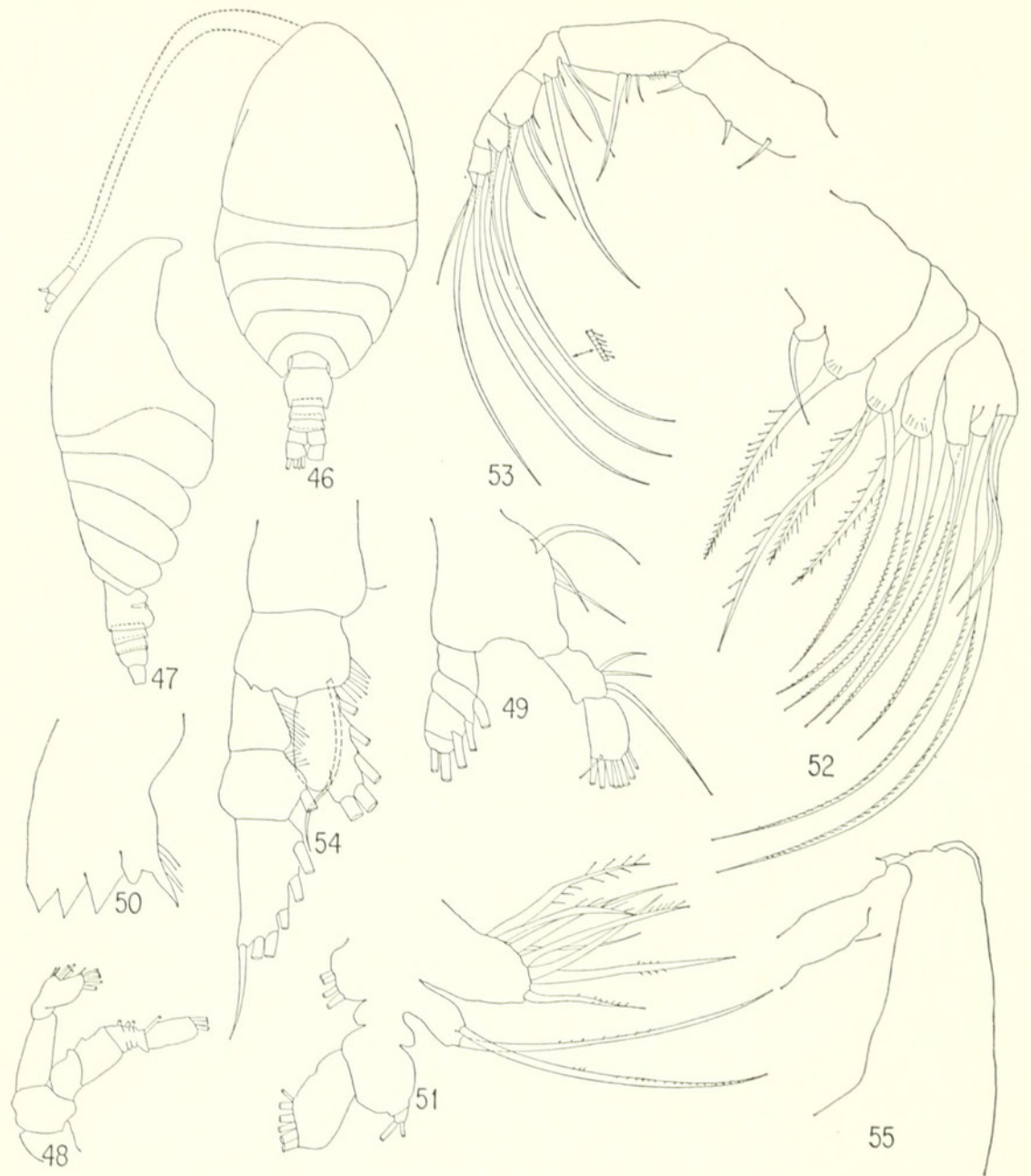
FIGURES 46-55.— Bradyetes florens , new species, female: 46, dorsal view; 47, lateral view; 48, second antenna; 49, mandible palpus; 50, mandible blade; 51, first maxilla; 52, second maxilla; 53, maxilliped; 54, first foot. Chirundinella cara , female: 55, head, lateral view.
