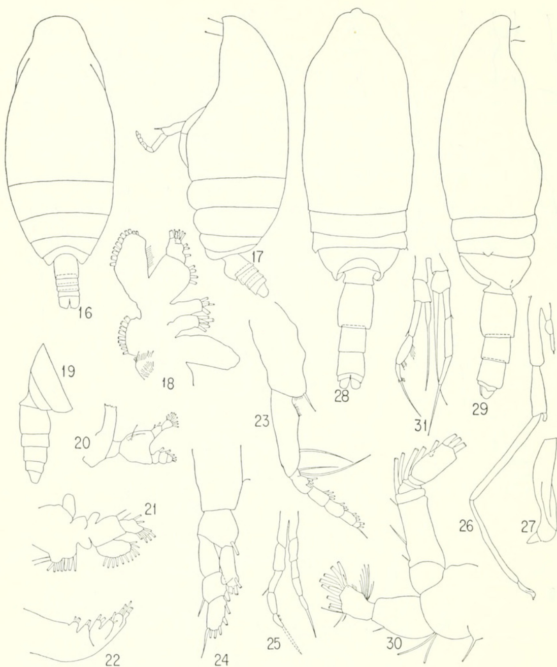
FIGURES 16-31.— Mimocalanus inflatus ?, female: 16, dorsal view; 17, lateral view; 18, first maxilla (spines on inner lobe omitted). Mimocalanus species, male: 19, posterior end of thorax and abdomen, lateral view; 20, mandible; 21, first maxilla; 22, second maxilla; 23, maxilliped; 24, first foot; 25, fifth feet. Spinocalanus longipes , male: 26, fifth feet; 27, terminal segment of left fifth foot. Spinocalanus validus , male: 28, dorsal view; 29, lateral view; 30, second antenna; 31, fifth feet.
