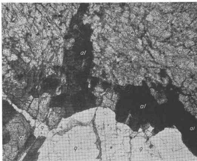
FIG. 10. (125 \times ) Photomicrograph of cerite specimen from southern deposit, showing the border of a large veinlet of allanite (al), and quartz (q) that cuts through the cerite (c). Arrows point to minute spots of uraninite.
