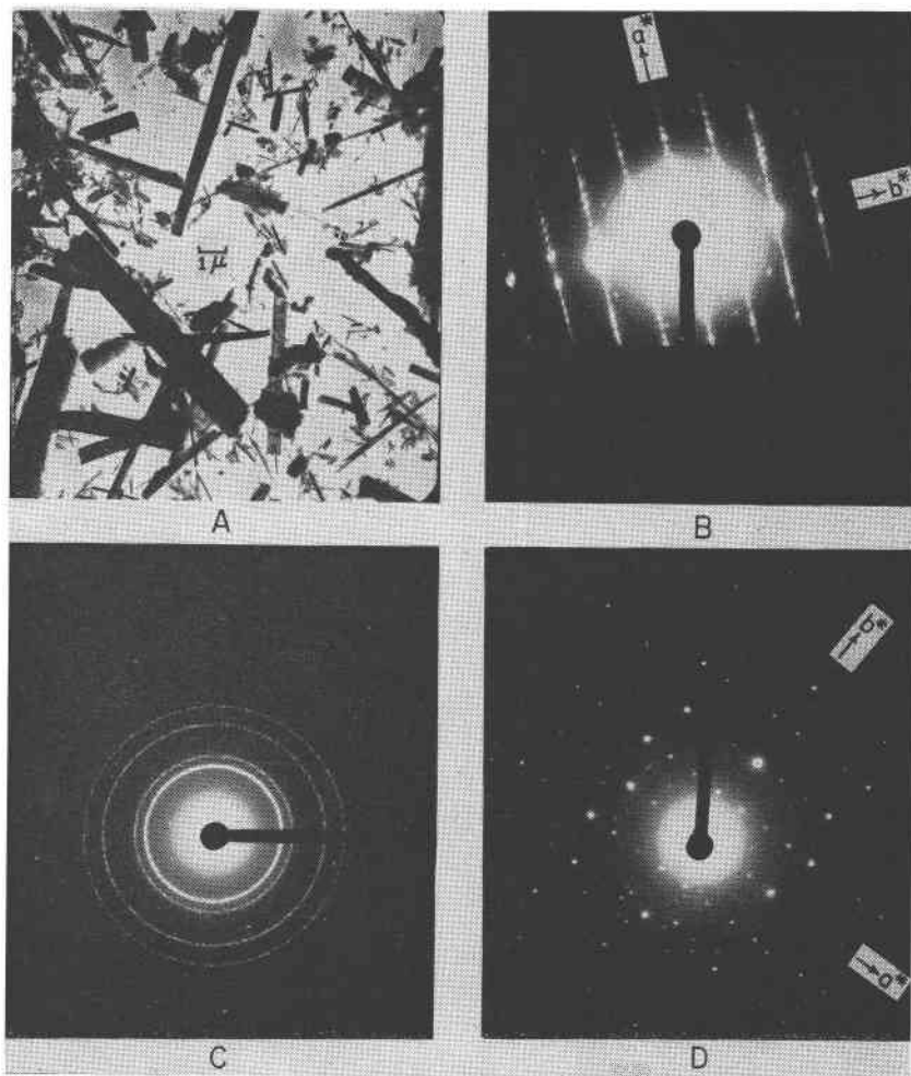
FIG. 7. Electron micrograph and diffraction patterns of navajote and a "corvusite-like" material associated with navajote. (A) Electron micrograph of sample A. (B) SAD spot pattern of navajote. (C) Aluminum standard. (D) SAD spot pattern of a "corvusite-like" mineral associated with navajote.
