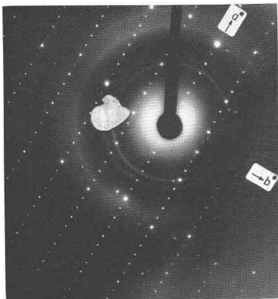
FIG. 4. SAD spot pattern of a new hydrated calcium vanadyl vanadate from the J. J. mine superimposed on the powder pattern of the internal aluminum standard.
