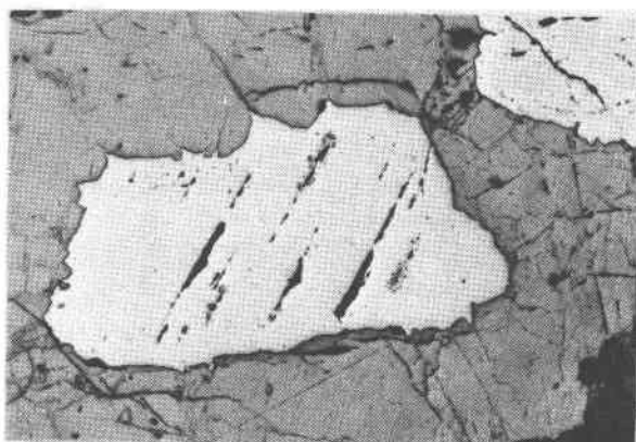
Fig. 2. Bright pyrrhotite, interpreted as a residual cusped island being replaced by bartonite. 77-CYP-31, 1.06 \times 1.50 mm.
