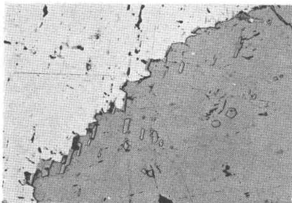
Fig. 3. Concentration of sharply bounded, fine-grained magnetite along interface between pyrrhotite (bright) and bartonite, 77-CYP-31, 0.72 \times 1.00 mm.
