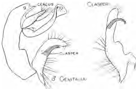
Fig. 90. Athripsodes alagmus
