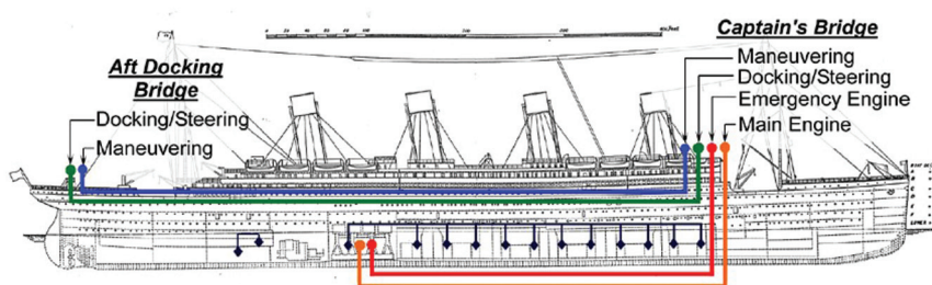
Engine Room Titanic's docking telegraphs
