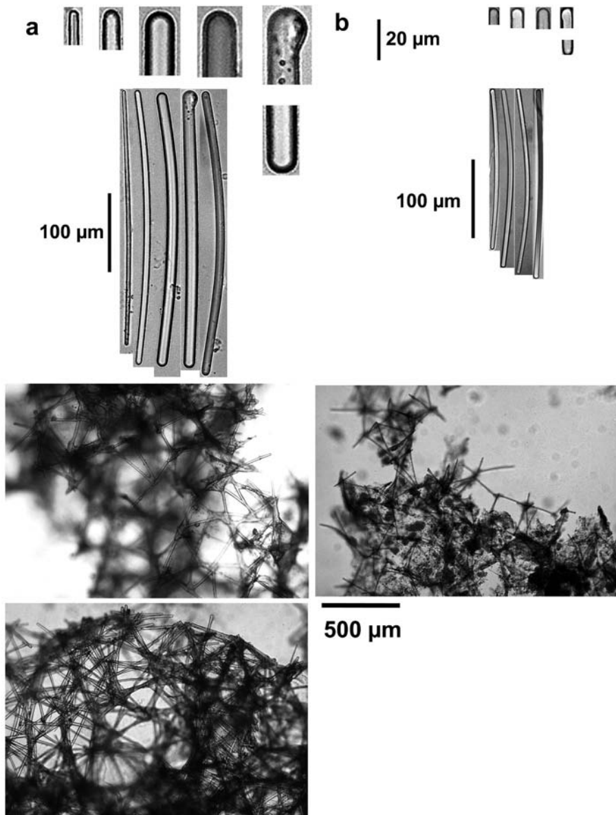
Figure 4. Microphotographs of the skeleton of Xestospongia deweerdtae comparing free living (a, left) and Plakortis -associated (b, right) studied specimens from the Bahamas. From top to bottom, spicules (upper panel), tangential view of the ectosome (middle panel), and perpendicular section of the choanosome at the surface (lower panel). Notice the marked differences in size of spicules for the two forms in the same geographical area.
