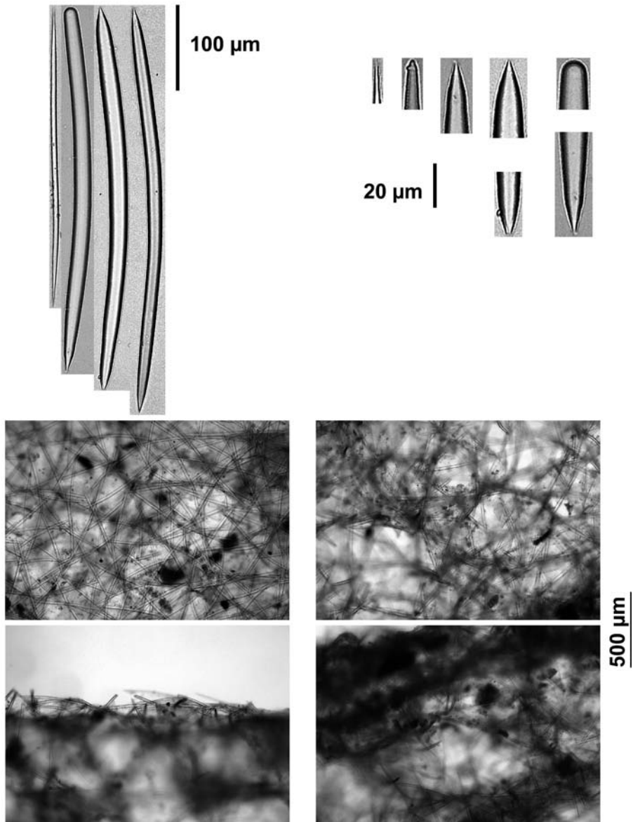
Figura 3. Microphotographs of the skeleton of Xestospongia arenosa of the studied material from Santa Marta. From top to bottom, spicules (upper panel), tangential view of the ectosome (middle panel), and perpendicular section of the choanosome at the surface showing the ectosome and the upper choanosome (lower panel).
