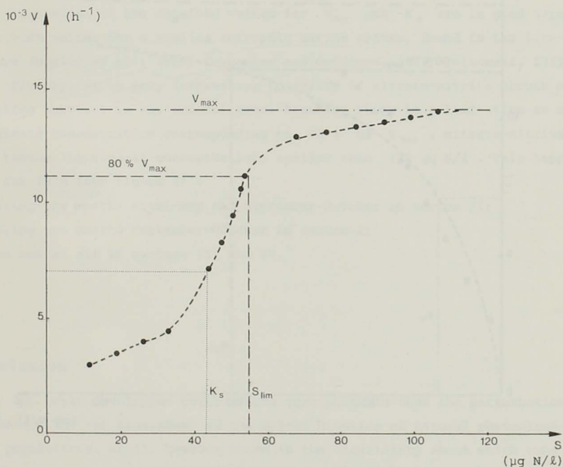
fig. 7. Uptake rate versus substrate concentration Experiment IV A
