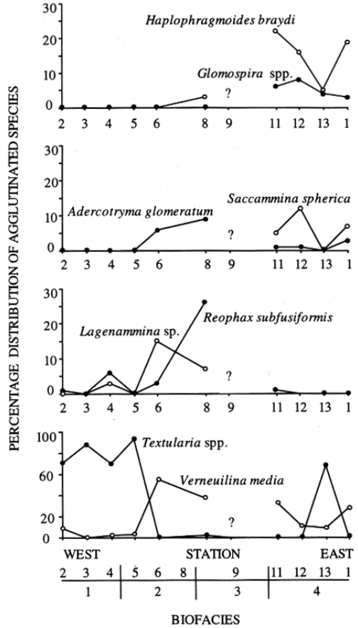
Fig. 3: The percentage distribution of the most common agglutinated species at each station. The questionmark (?) at Stn 9 indicates that percentage calculations were not carried out due to a low number (12) of agglutinated specimens.
