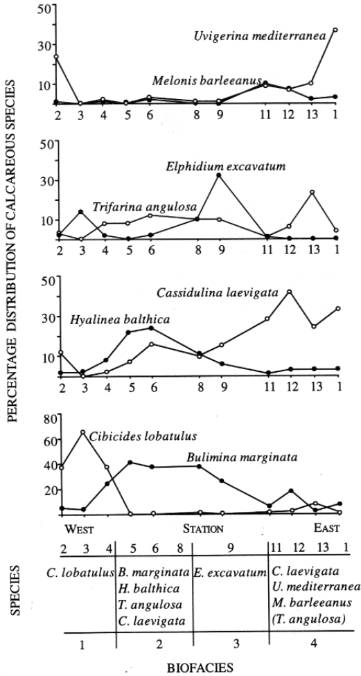
Fig. 2: The percentage distribution of the most common calcareous species at each station. Also shown are the common species and stations included in each biofacies. Trifarina angulosa and Stn 13 are marked with parentheses ( ) in biofacies 4 because this sample is distinct from the Cassidulina laevigata -biofacies.
