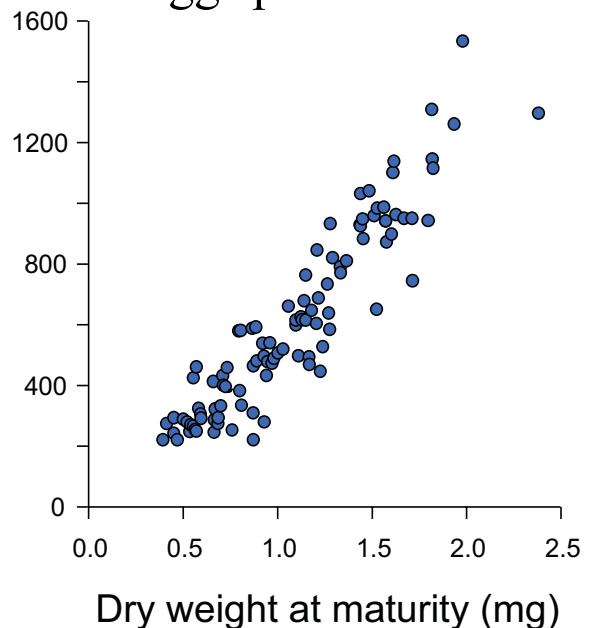
Fig. 17. Relationship between size (mg dry weight) of mature female larvae and fecundity (the number of eggs per female). (Modified from Peckarsky et al. 1993.)
