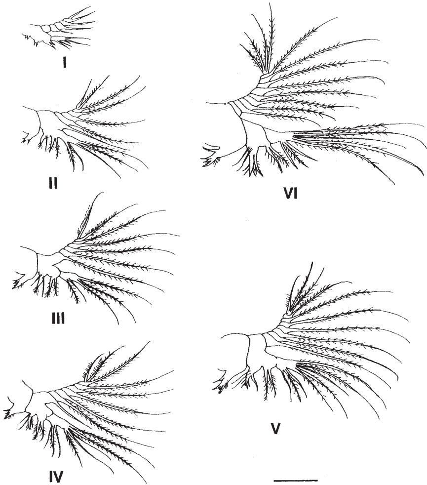
Fig. 5. Antennae of the six nauplius stages of B. reticulatus . Scale bar = 100 \mu m.
