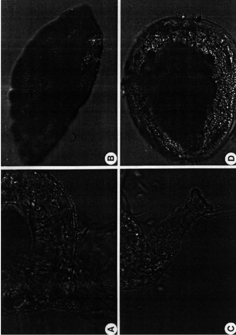
Fig. 7. Nauplius, cyprid and young adult of Breticulatus . (A) Lateral margin of the cephalic shield with numerous small spines in nauplius of stage II. (B) A cyprid with numerous small denticulate processes on the carapace surface and with a median eye. (C) Antennule of the cyprid terminated in the fourth segment. (D) Juvenile young adult with compound eyes in front of the anterior region.
