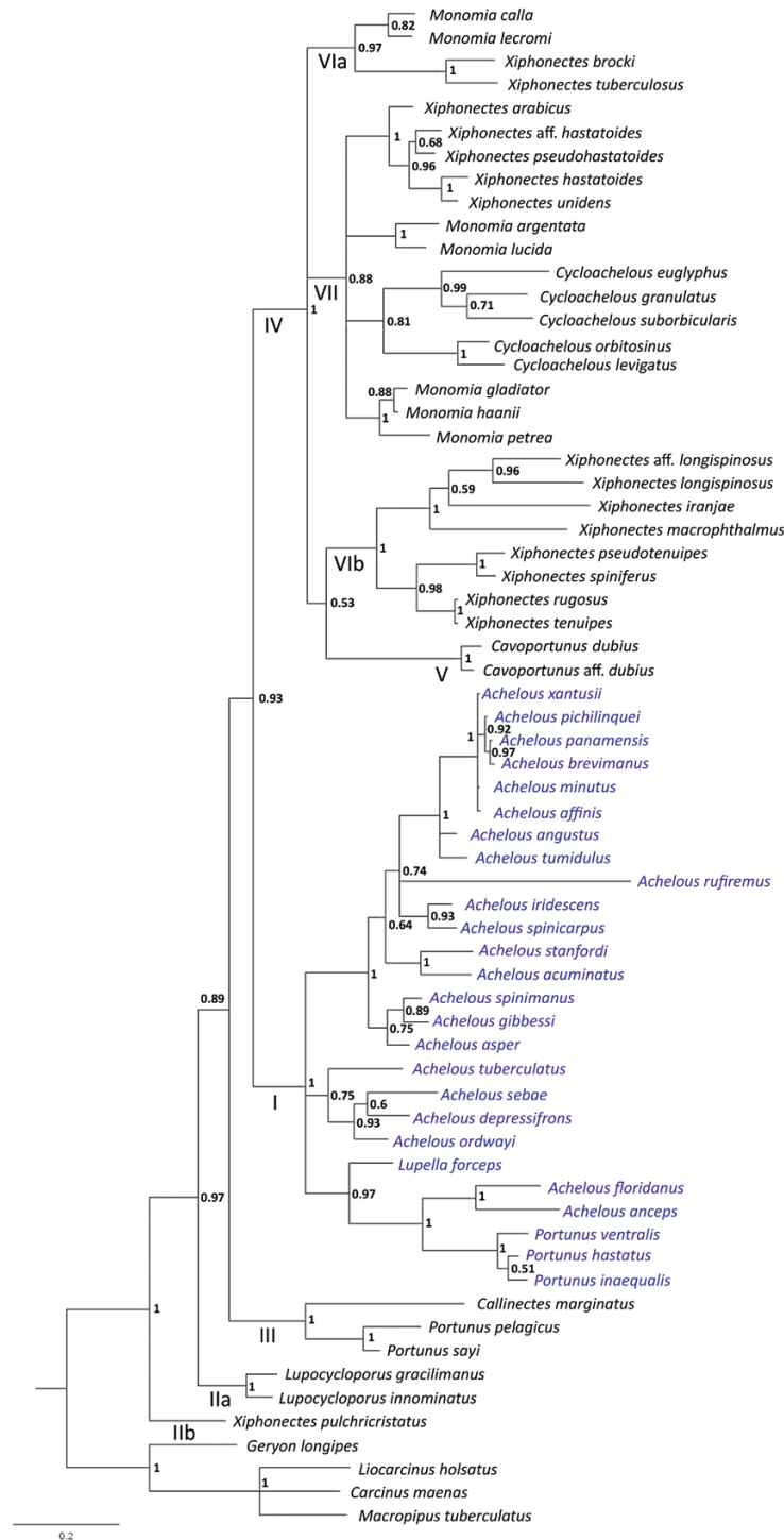
Figure 2. Bayesian phylogeny inferred from partial sequences of 16S rRNA mitochondrial gene. Posterior probabilities are shown at internodes. The blue colour of taxa names indicates geographical (Atlantic and eastern Pacific) affiliation comprising actual species in the genus Achelous .
