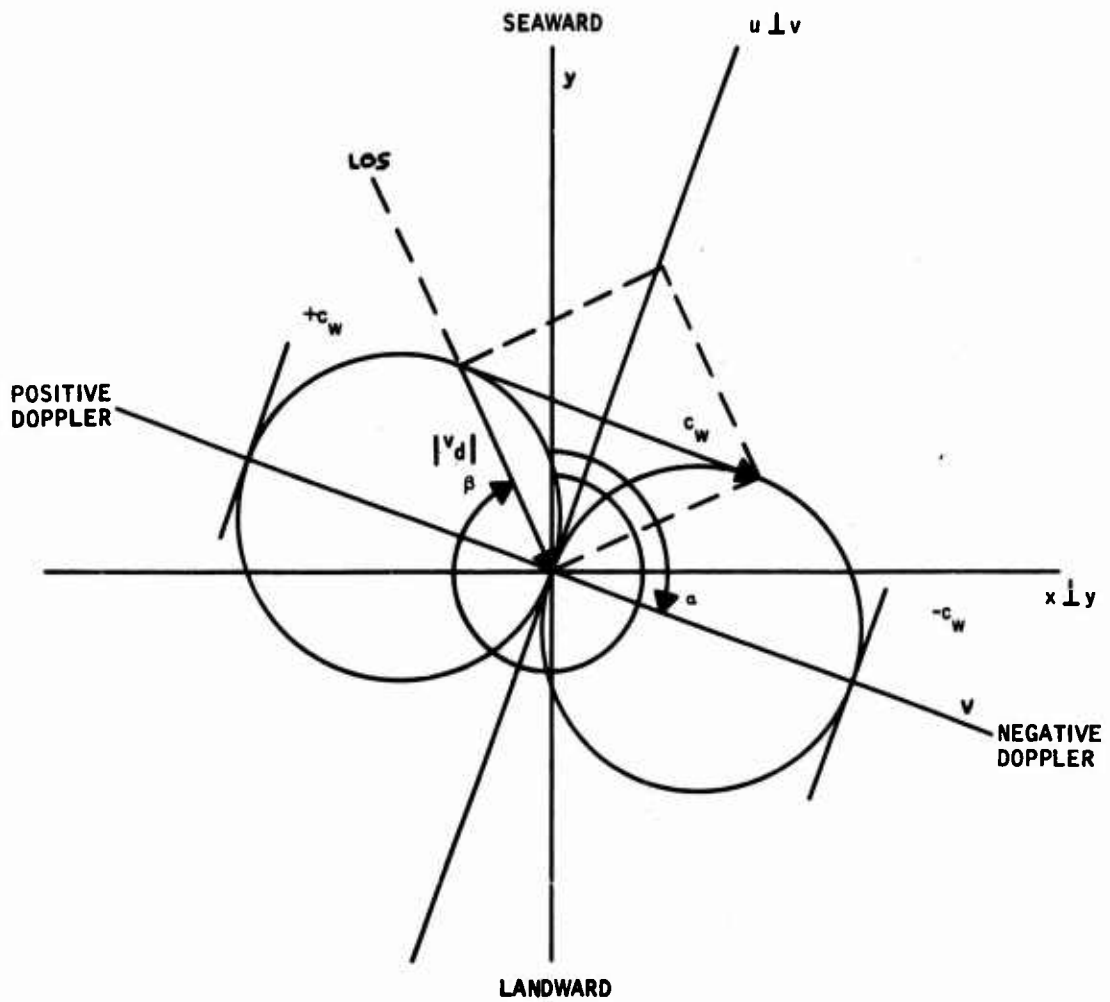
Figure 10. Doppler Geometry
