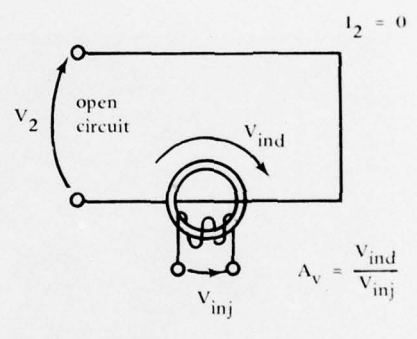
(b) Equivalent circuit for determining transfer function A_v .
