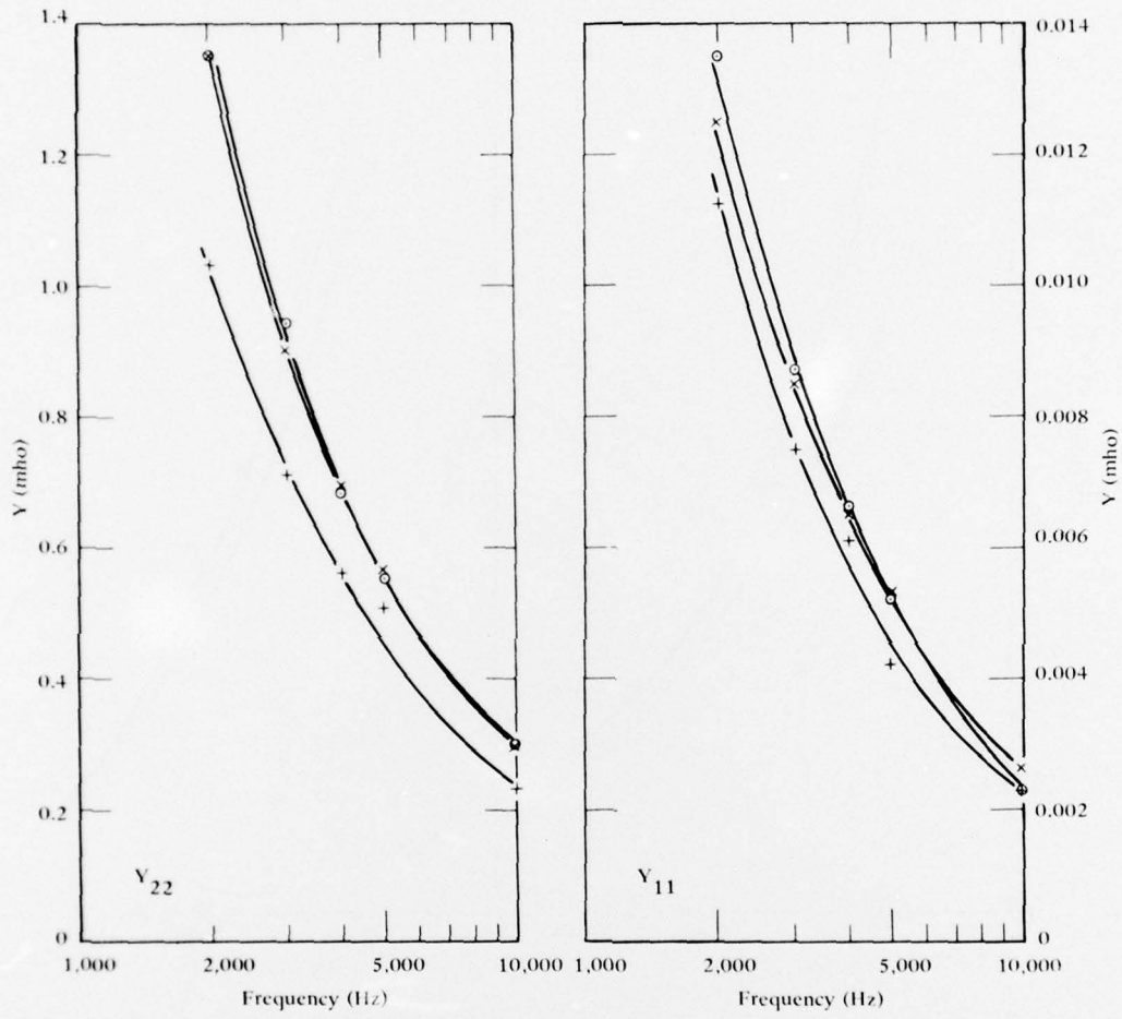
(a) Y_{22} versus frequency using different measurement methods.
