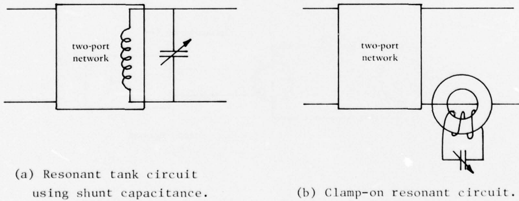
Figure 2. Simulated open circuits using resonant circuits.
