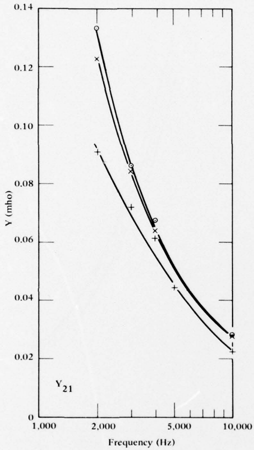
(c) Y_{21} versus frequency.
