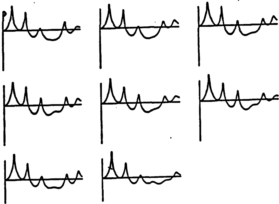
Figure 7. Frequency plot (FPL) of 8 frames of an adult male speaker's spectral tilt variations during the production of (a) phonated /ʌ/ and /b/ whispered /ʌ/.
