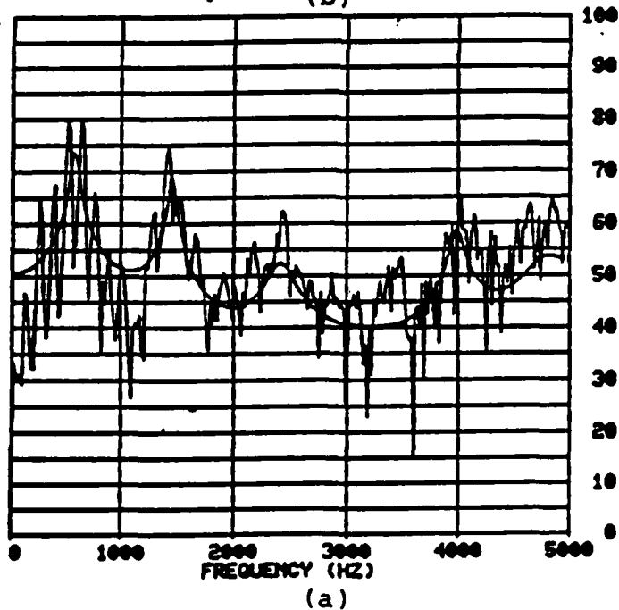
Figure 10. An FFT raw spectrum (FDI) and smooth spectrum (SSP) of an adult male's (a) phonated and (b) whispered production of the vowel /ʌ/.
