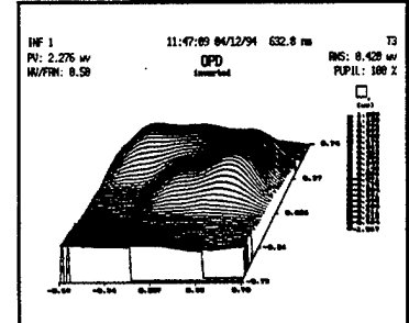
▲ Data sheet showing random distortions in MRL's deformable mirror.
