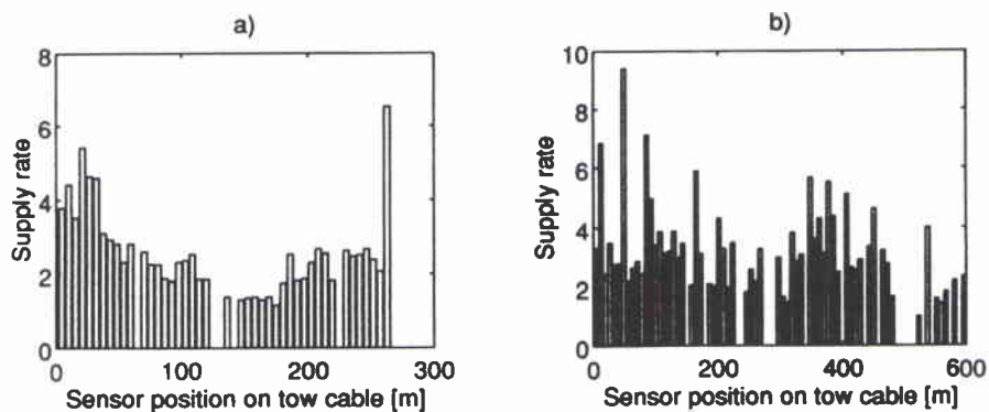
Fig. 4. Supply rates of sensors aligned on a CTD chain. A supply rate of n indicates that the sensor power supply needs only 1/n of supply time to fill the storage capacitor. A missing bar means that the sensor did not respond. (a) The 270 m chain was directly coupled to the sea water at its lower end.
