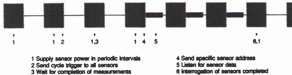
Fig. 3. Communication between deck unit and sensors. Periodic send and receive intervals are maintained during a data cycle.
