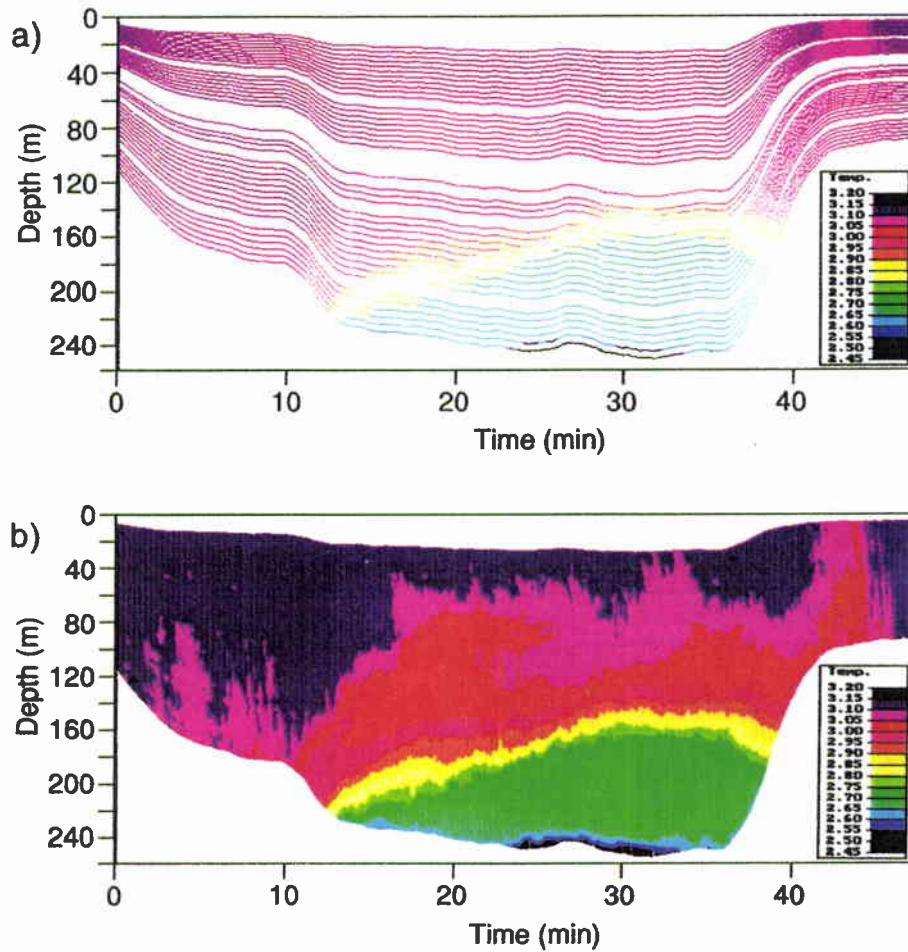
Fig. 5. Temperature section in the Norwegian Sea at 73^{\circ}30'N 6^{\circ}50'E in February 1993. The towing ship slows down and is almost stationary for 12 min when the downmost sensors reach 245 m; it then speeds up to 8 kn again. (a) Every coloured pixel represents the average of two consecutive temperature measurements. The pixels are colour-coded according to the temperature scale on the right. Missing sensors were destroyed in an emergency manoeuvre. (b) Data are linearly interpolated in the vertical direction.
