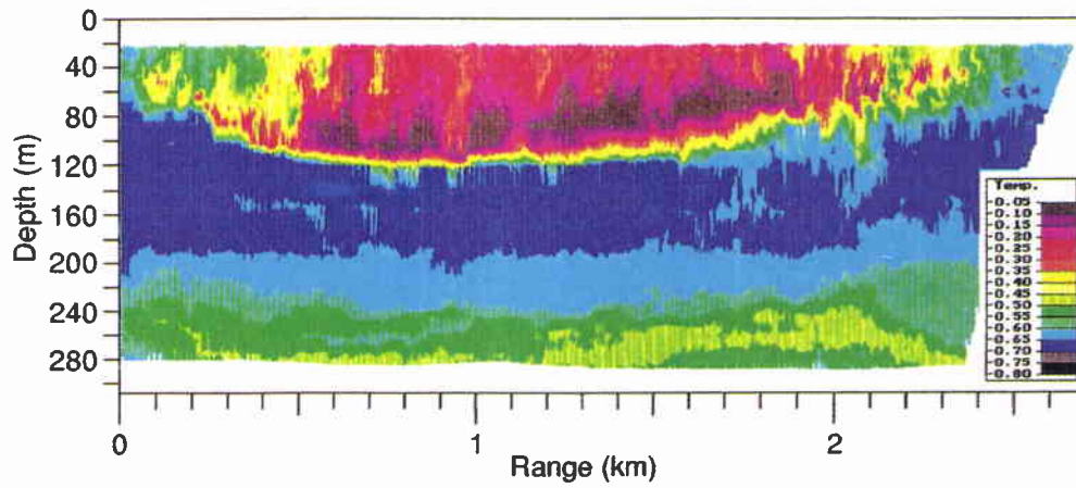
Fig. 7. Lens of warmer (by 0.5^{\circ}\text{C} ) and more saline (by 0.04 units) water in the surface layer of the Greenland Sea in March 1994, which is eroded by mixing and heat flux to the air. Wind speed is about 8\text{ m s}^{-1} , air temperature -9^{\circ}\text{C} .
