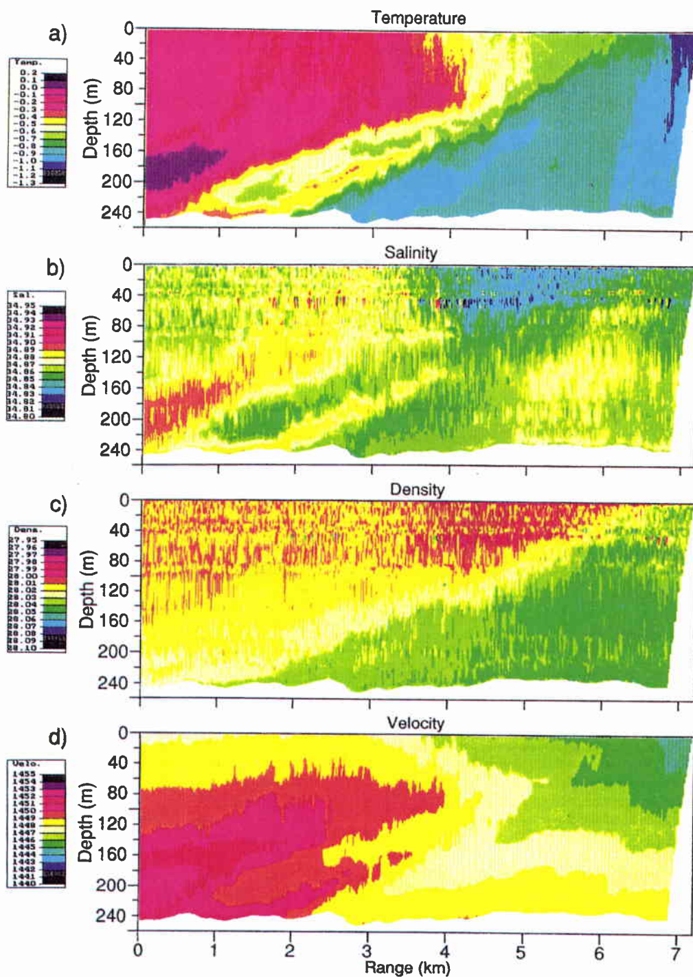
Fig. 6. Boundary of a patch or tongue of advected water in the Greenland Sea. (a) Temperature, (b) salinity, (c) density, (d) sound velocity. The intermediate temperature maximum at the cold water interface is balanced by salinity and has no corresponding density.
