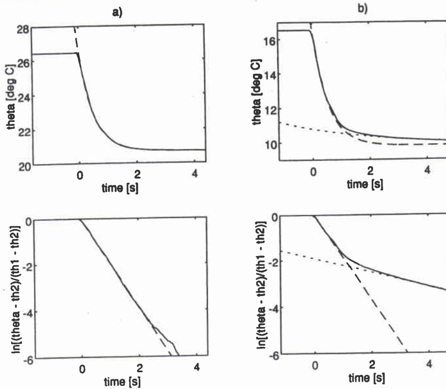
Fig. 1. Response of temperature sensors to a thermal jump. The time constant is approximately 0.5 s in both cases. Dashed curves are theoretical responses of an ideal temperature sensor. (a) Response of a CTD chain sensor. (b) Thermal coupling between sensing element and carrier inhibits fast transition to end temperature. The time constant of the carrier is 3.3 s in this case (dotted curves). This sensor design was rejected.
