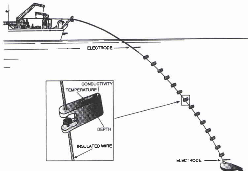
Fig. 2. Diagram of the CTD chain. The sensors are inductively coupled to the towing cable. The current loop is closed by sea water.
