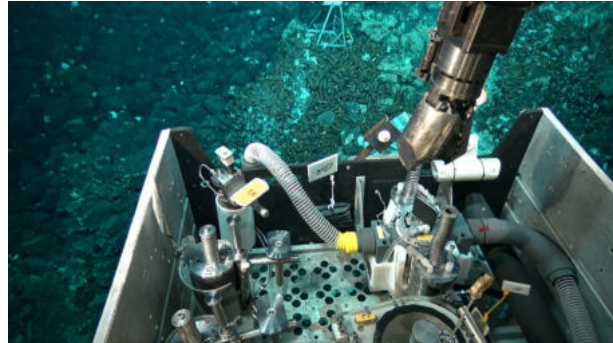
Figure 72 : FISH system inside the ROV basket
