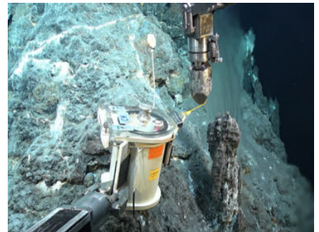
Figure 8: Sampling CH6, opening the BioBox close to the vent
