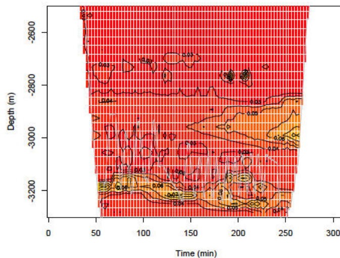
Figure 3: Turbidity anomalies along CTD01 profile. The grey line is the towpath of the CTD-rosette.
