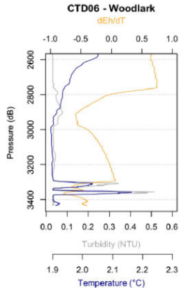
Figure 8: Turbidity, Eh and Temperature anomalies over the CTD06 station, near TVG150 in the vicinity of an active vent.
