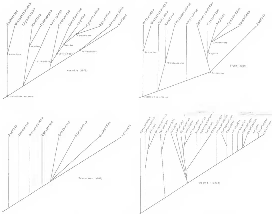
FIG. 4. Some evolutionary trees from previous studies, by Kussakin (1979), Bruce (1981), Schmalfluss (1989), and Wägele (1989a).
