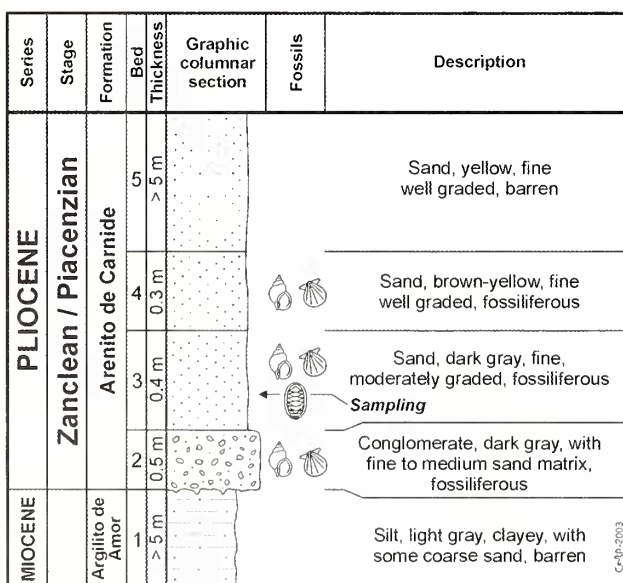
Fig. 2: Stratigraphy of the Vale de Freixo section
