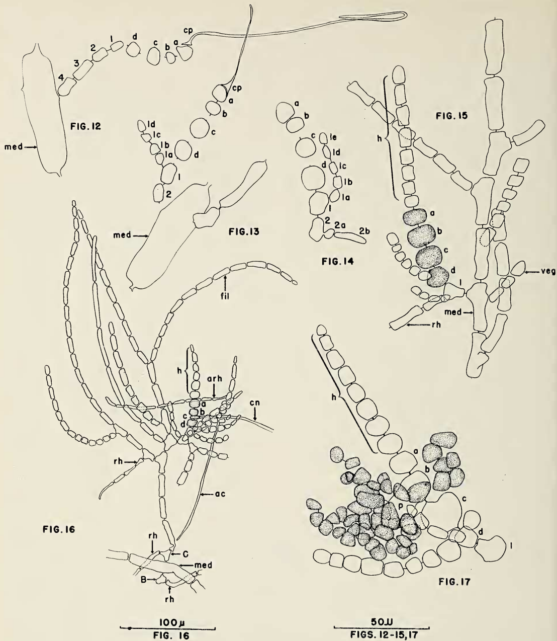
FIGS. 12-17. Microscopic sexual reproductive features of Gibsmithia hawaiiensis . The specialized cells, a-d , are similar in nature whether in a carpopogonial or auxiliary-cell branch. On the latter, the piliform extension, b , shows as a multicellular hair, the cells of which are in staining reaction and appearance, rather like vegetative cells of similar size and relative terminal position elsewhere. 12-14, Carpopogonial branches with or without nonfertilized carpopogonia, cp . The hypogynous cells a-d were always densely granular and their contents took up aniline-blue from aqueous solution much more than did the other nearby cells. Cell b was usually smaller and the contents were usually different from the rest. Cell c was almost always the largest. The numbered cells, 1, 2, 3, etc., represent cells that looked like the strictly vegetative cells of similar size and position nearby and connected the carpopogonial branch to a medullary cell, med . The cytologically similar cells of the sterile branchlets are indicated as 1a , 1b , 1c , etc. (Collection No. 10386.) 15, A nonfertilized auxiliary-cell branch arising from one of two opposite branch systems of the same medullary cell, med , the one vegetative branch system, veg , being of only three cells, the other more extensive and bearing an auxiliary-cell branch.
