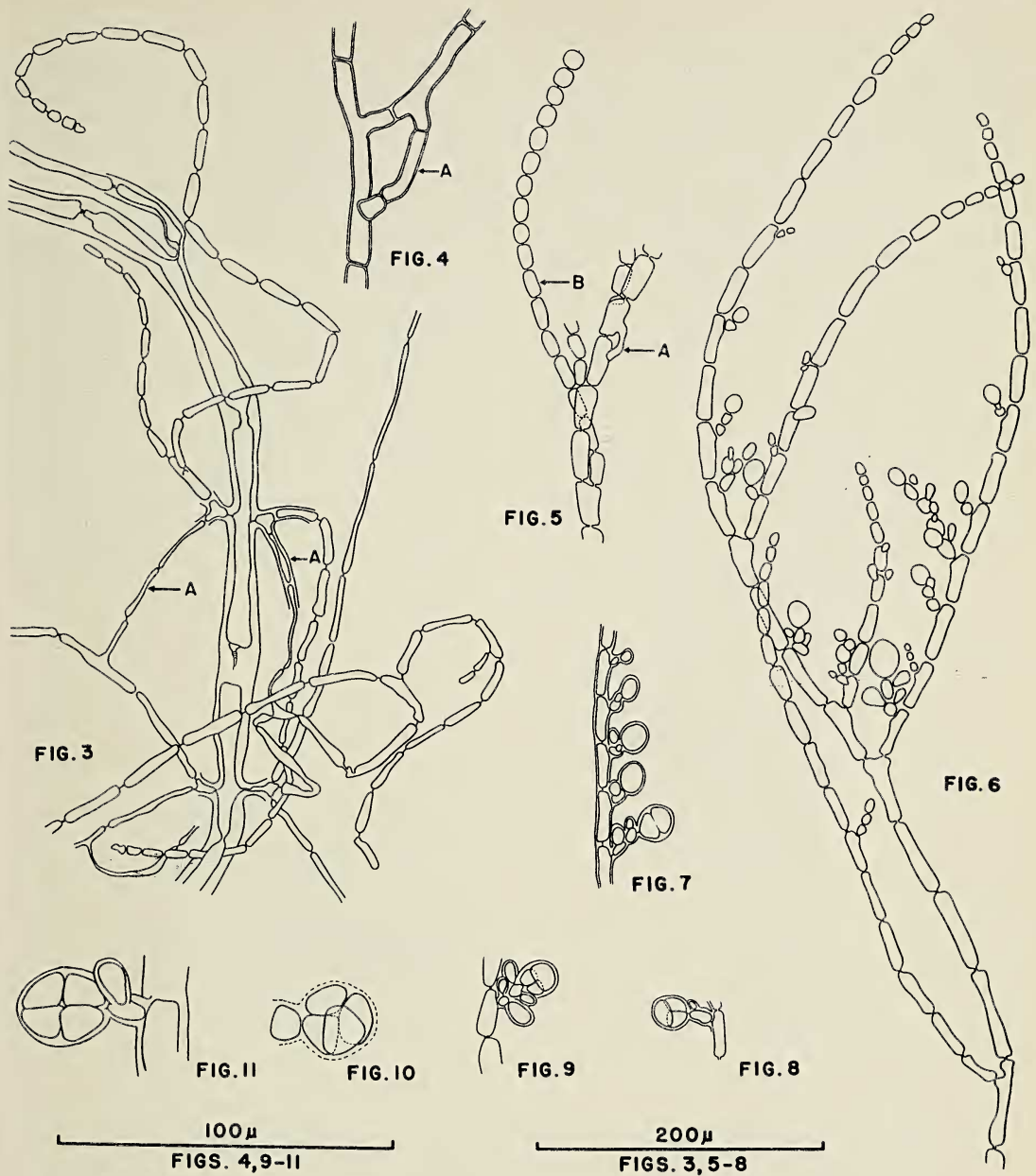
FIGS. 3-11. Vegetative and asexual reproductive microscopic structural details of Gibsmithia hawaiiensis (collection No. 12343). 3, An axial filament from the medullary region of a gelatinous branch of the thallus showing the opposite ramification of the medullary filaments and, A , characteristic reconnecting rhizoidal branches. 4, A more simple reconnecting rhizoidal branch, A , from one of the subdichotomous cortical filaments. 5, A seiospore-bearing ultimate branchlet on a subdichotomous cortical filament with, A , a very simple reconnecting filament or rhizoid. Such lateral nonbranched filaments, B , with a terminal series of seiospores were found arising from almost every second cell in the vegetative axis of this part of the filament system. The origins of but three such seiosporic branches are shown here. 6, A tetrasporangium-bearing cortical filament system. Divisions within the tetrasporangia are not shown and no attempt was made to represent all pit connections. 7-11, Tetrasporangia in various stages of maturity. The arrangement of spores is always at first cruciate but, as indicated by Figure 10, in age they may not be in a strictly cruciate arrangement.
