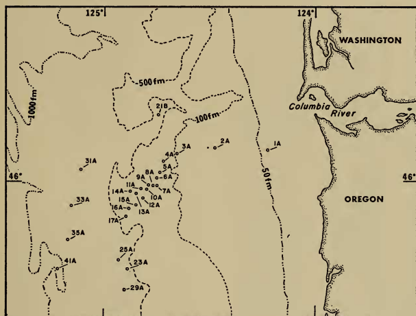
FIG. 1. U. S. Bureau of Commercial Fisheries-Atomic Energy Commission trackline study area off the northern Oregon coast, showing approximate trawling station locations of M/V Commando and John N. Cobb , 1961-1964, from 50 to 1050 fathoms (91 to 1920 meters). (Prepared by Miles S. Alton.)
