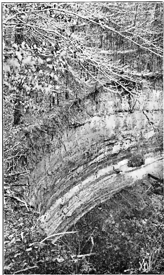
WILCOX FORMATION. Patroon Bayou, Sabine County.
