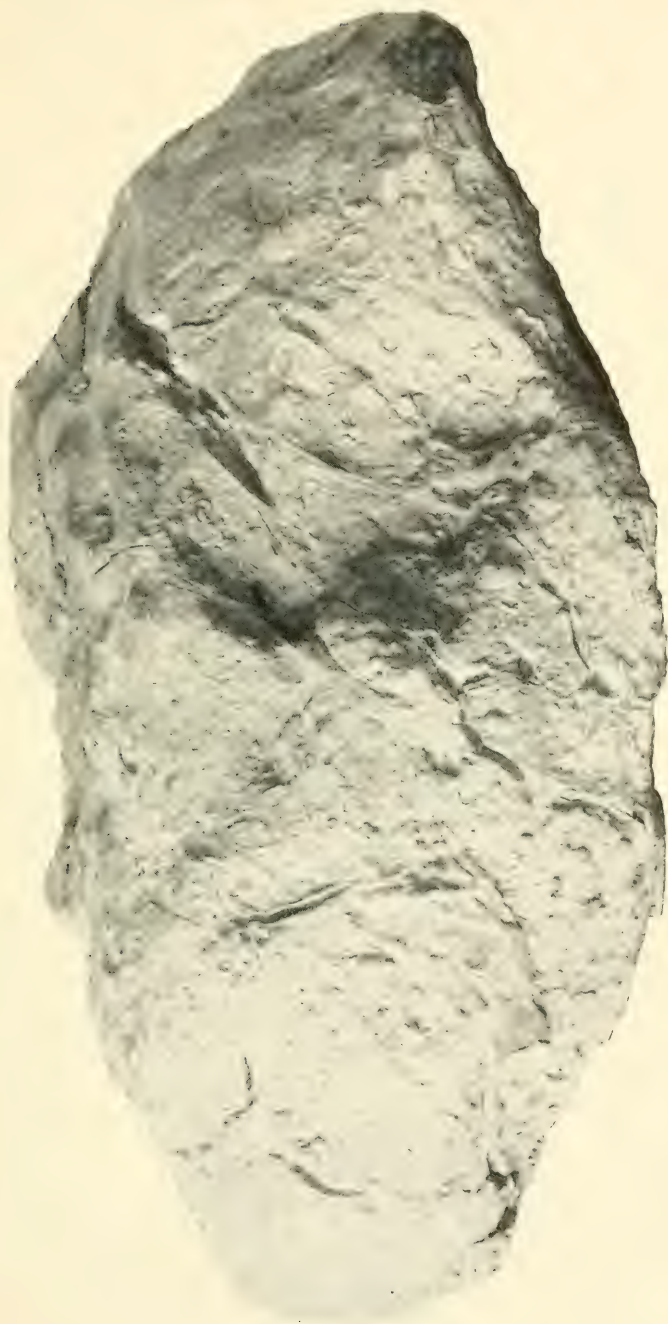
The main mass of the Sardin meteorite. This is so deeply weathered that there is almost no external evidence to suggest that it is a meteorite.
