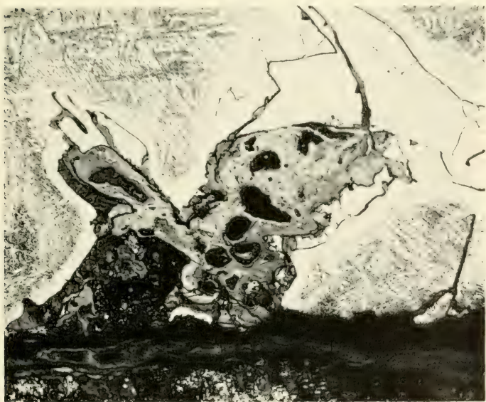
2. Invasion of oxide into the kamacite. Picral etching. \times 100 .
