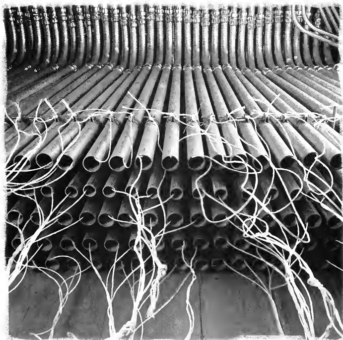
This is the electrical "nerve center" of the new science building. Pictured is just a small portion of the seven miles of conduit that run throughout the building.
