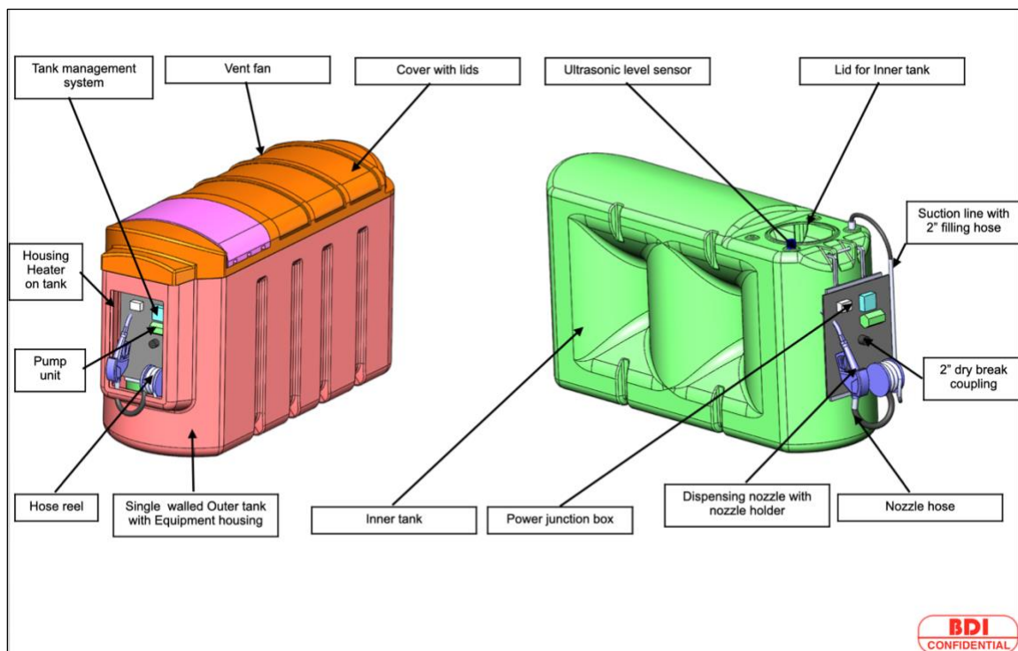
AdBlue Kingspan tank 2,000 liters with dispensing equipment
