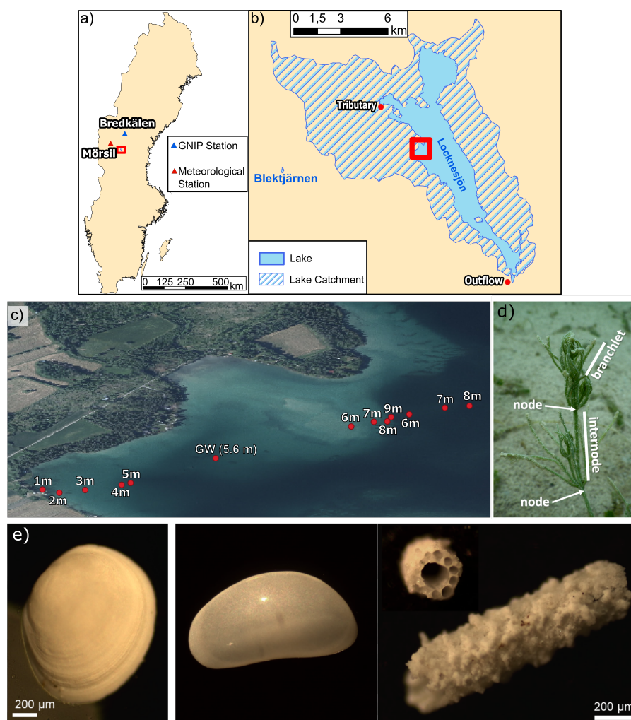
Figure 2. (a) Map of Sweden showing the location of the study area (red rectangle), of the GNIP station Bredkålen and of the meteorological station Mörnsil. (b) Lake Locknesjön with its catchment (hatched) and Lake Blektjärnen. (c) Locations of the sampling sites on a transect from the shore towards the center of the lake. The area shown in (b) is marked by the red rectangle in (a) and the area shown in (c) is marked in (b) (country outline from USGS, lake and catchment outline from SMHI, 2020a; orthophoto © Lantmäteriet 2020). (d) Photograph of a Chara hispida in Lake Locknesjön. An internode (between two nodes) and a branchlet are indicated on the image. The part of the Chara hispida visible on the photograph measures about 2 cm in height. (e) Images of different lacustrine biogenic carbonates analyzed in this study: (left) Pisidium valve, (middle) adult Candona candida valve, (right) Chara hispida encrustations.
