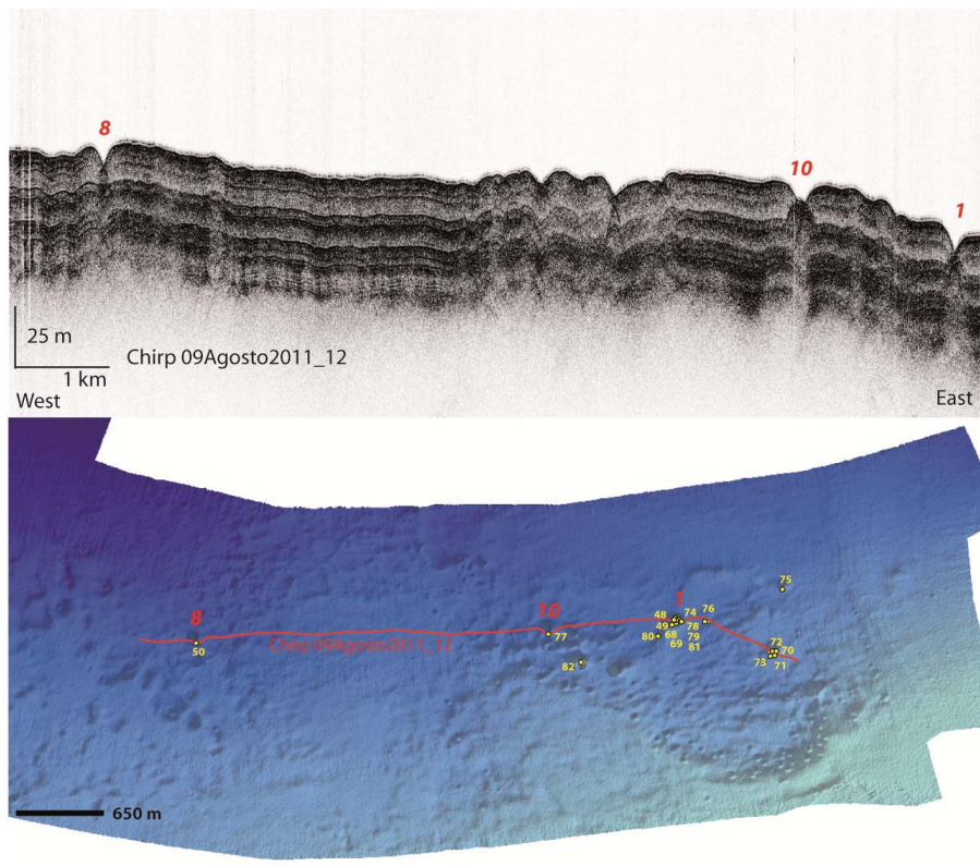
Fig. 5. (A) Chirp profile showing the subsurface stratigraphy of the pockmark area; (B) 3-D perspective view of the DTM shows the location of the chirp profile and the sample locations.; MEDCOR samples yellow, DECORS samples red.
