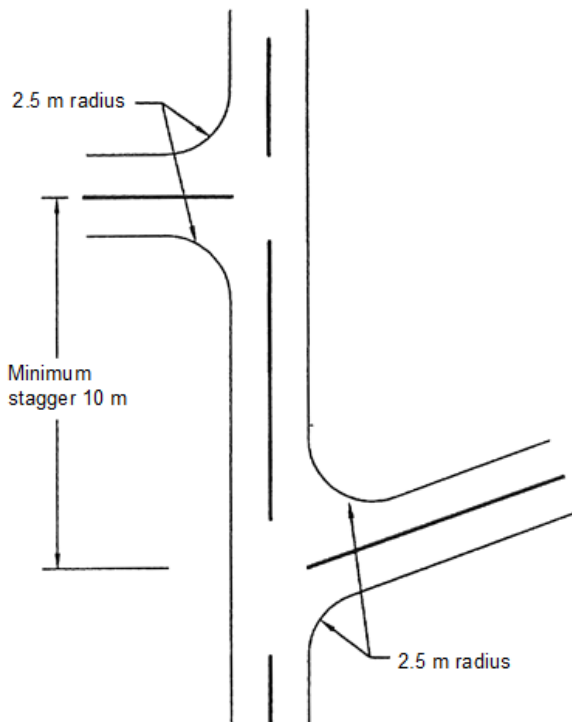
Figure 6.5: Example of a staggered T-intersection
