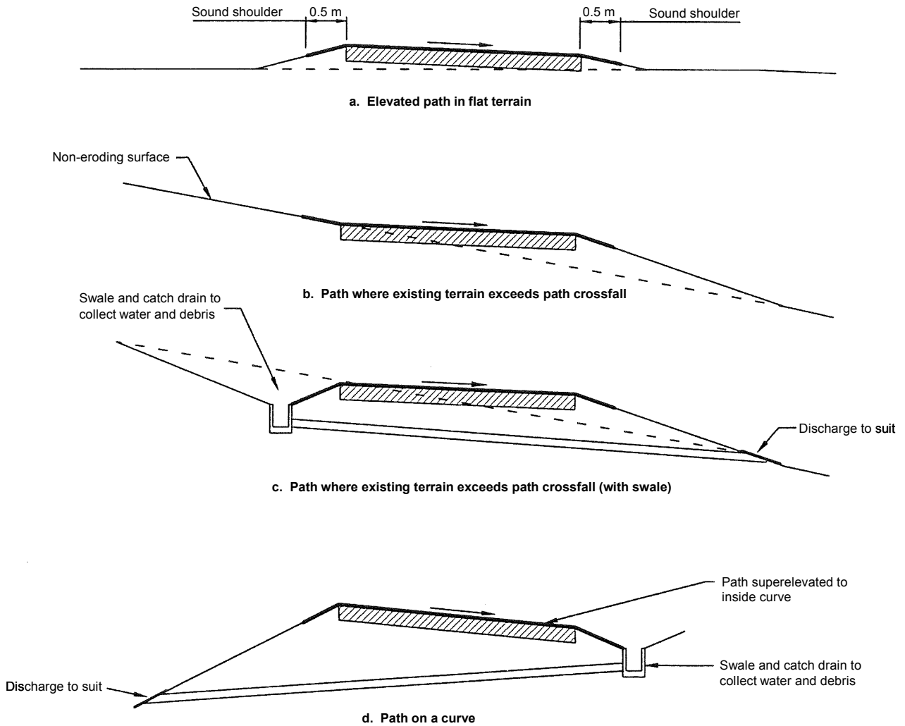
Figure 5.14: Drainage and crossfall requirements
