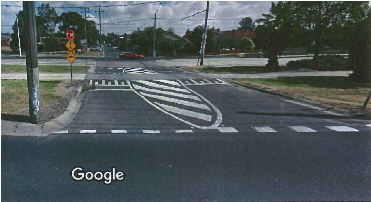
Figure 4.1: Example of a median path at a road crossing
