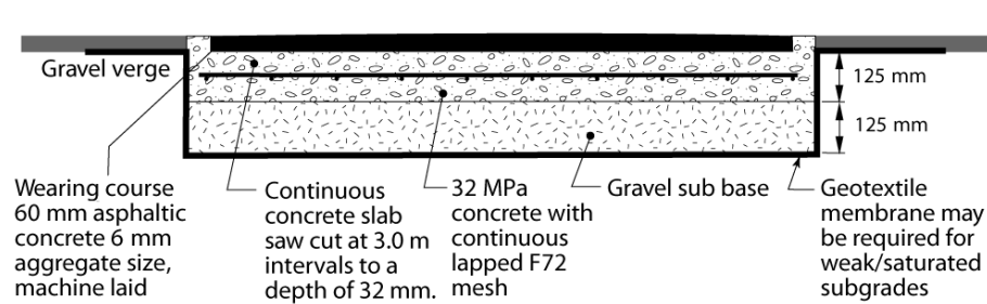
(a) Reinforced concrete path with asphalt surface and gravel sub base
