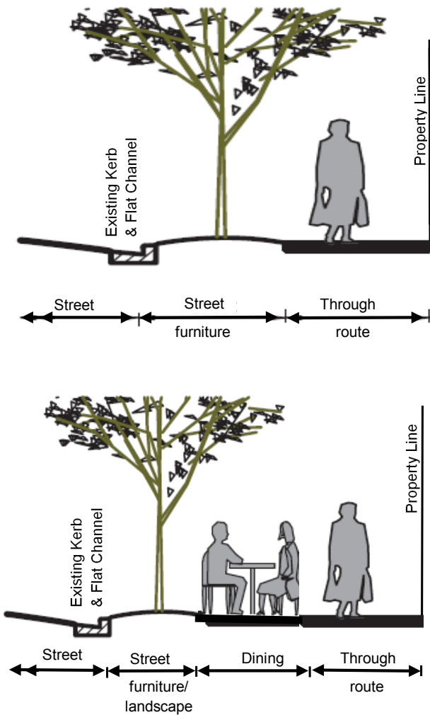
Figure 2.1: Examples of pedestrian path zones
